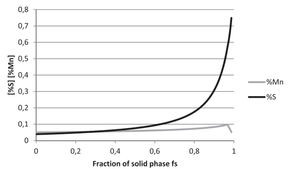
Fig. 7. Microsegregation of Mn and S during solidification of steel no. 1 at the cooling rate of 500K/min for steel no.1. MnS activity in precipitations equals to 1
