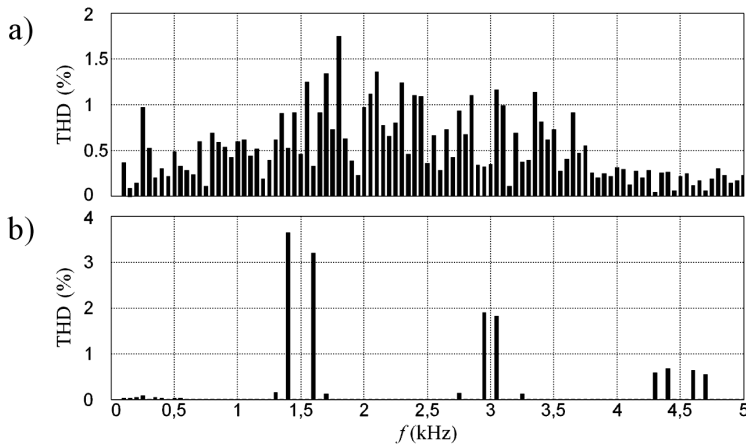
Figure 10. Spectrum of current higher harmonics of the PWM rectifier working with: a) the HCC method, b) the sinusoidal PWM method; the first harmonic is not shown, switching frequency was equal to 1500 Hz.
