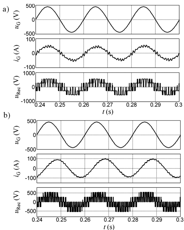
Figure 5. Generator output phase voltage u_G and current i_G , and input phase voltage u_{Rec} of the PWM rectifier: a) \varphi = 0^\circ , \psi = 9.7^\circ , b) \varphi = 60^\circ , \psi = 12.5^\circ .
