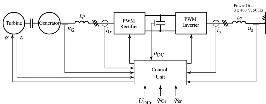
Figure 1. Energy conversion system with the PWM rectifier for a small water or wind plant: U_{DCr} – assumed voltage of the DC link, i_s – output current of the PWM voltage source inverter, u_s – voltage of the power grid, \varphi_{Gr} , \varphi_{sr} – assumed phase angle of the generator and output current respectively, u_G , i_G – voltage, and current of the PM generator, v – speed of wind or water, \alpha – angle of the turbine blades.
