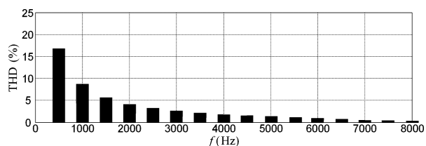
Figure 9. THD factor as a function of the assumed saw-tooth signal frequency in the sinusoidal PWM method.
