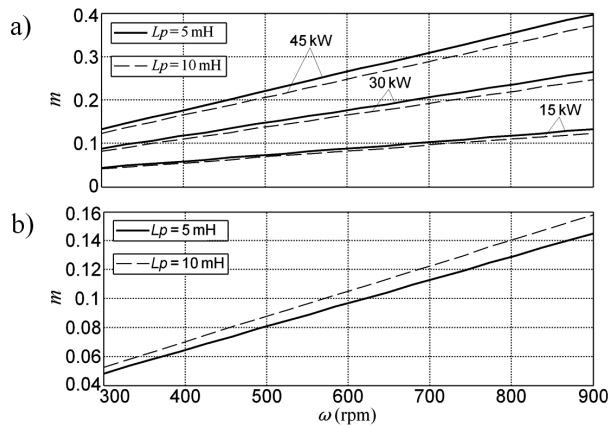
Figure 4. The coefficient m of the modulation depth as functions of the rotational speed \omega of the turbine – PM generator unit for assumed: a) power P ( \varphi = 0^\circ ), b) phase angle \varphi ( P = 30\text{kW} ).
