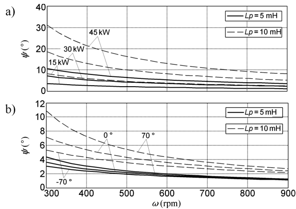
Figure 3. The angle \psi as the function of the rotational speed \omega of the turbine – PM generator unit for assumed: a) power P ( \varphi = 0^\circ ), b) phase angle \varphi ( P = 30\text{kW} ).
