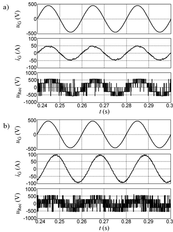
Figure 7. Generator output phase voltage u_G and current i_G , and input phase voltage u_{Rec} of the PWM rectifier controlled with the HCC method: a) \varphi = 0^\circ , I_{Gmax} = 50\text{A} , b) \varphi = 60^\circ , I_{Gmax} = 94\text{A} .
