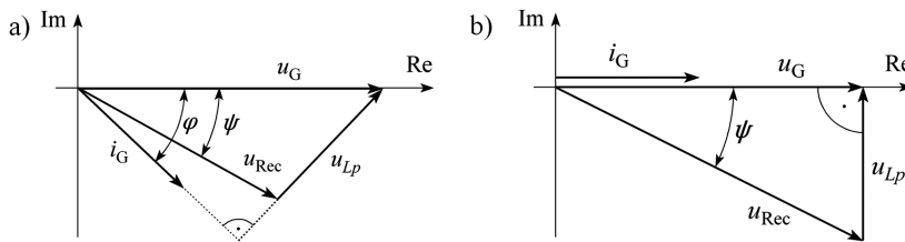
Figure 2. Phasor diagram in the PM generator – PWM rectifier system: U_G , I_G – output phase voltage and current of the PM generator respectively, U_{Rec} – input phase voltage of the PWM rectifier, U_{Lp} – voltage drop on the choke L_p .
