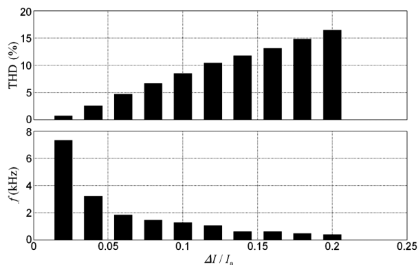
Figure 8. THD factor and average switching frequency as a function of the \Delta I/I_a value in the HCC method.
