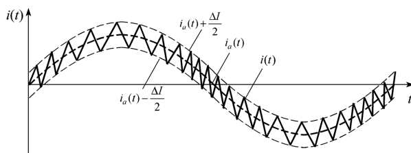
Figure 6. Phase current in the PWM rectifier controlled with the HCC method; i_a(t) , \Delta I – the assumed sinusoidal current waveform and value of the current changes respectively.
