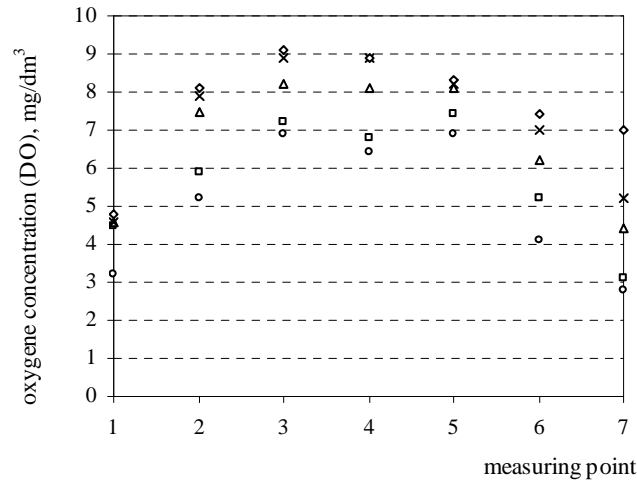
Fig. 4. Changes of DO in the sewage in 5 series
