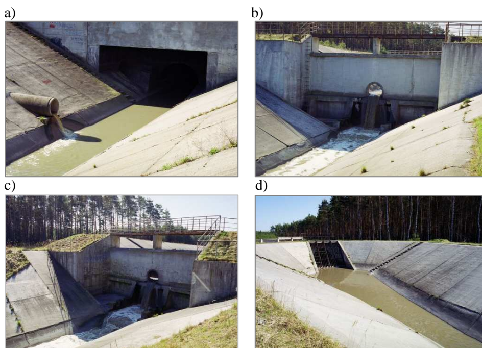
Fig. 3. View of the open sewer which channels sewage to WWTP in Lezyca a) beginning of the open sewer - measuring point 1, b) measuring point 2, c) measuring point 3, d) end of the open sewer - measuring point 7
