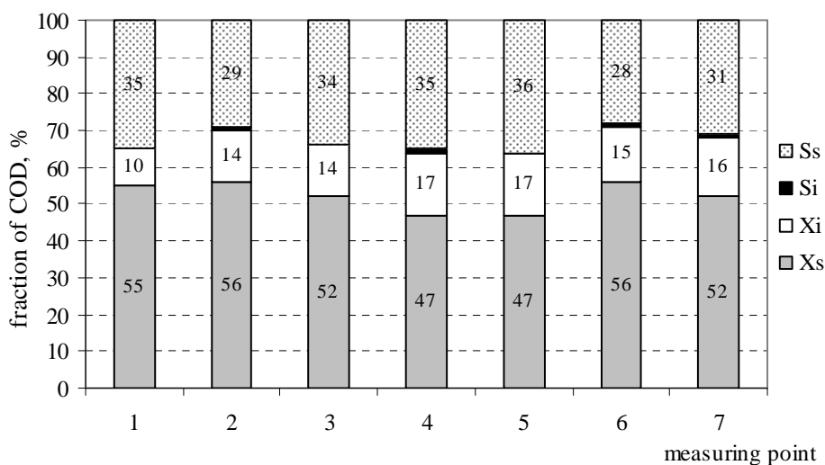
Fig. 6. Average values of COD fraction in the sewage at subsequent measuring points [divided into fractions in %]
