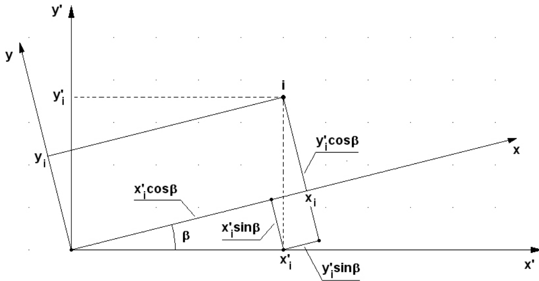
Fig. 6. Transformation of curve coordinates from the local system x'y' to the local system xy
