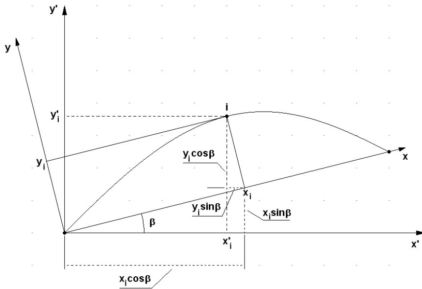
Fig. 3. Transformation of curve coordinates from the local system xy to the local system x'y'
