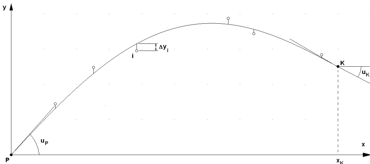
Fig. 5. A fitting of the general transition curve to the given direction points
