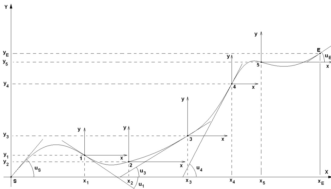
Fig. 2. Polynomial route created by general transition curves
