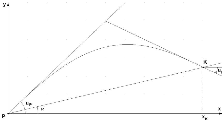
Fig. 1. The general transition curve in the local coordinate system
