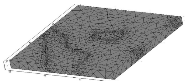
Fig. 2. Virtual 3D model of small slice of human bone identified by \mu\text{CT} method.
