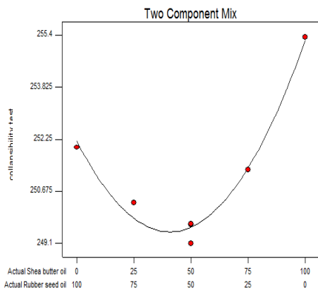
Fig. 46. 1.5% Oil in Sand: Collapsibility
