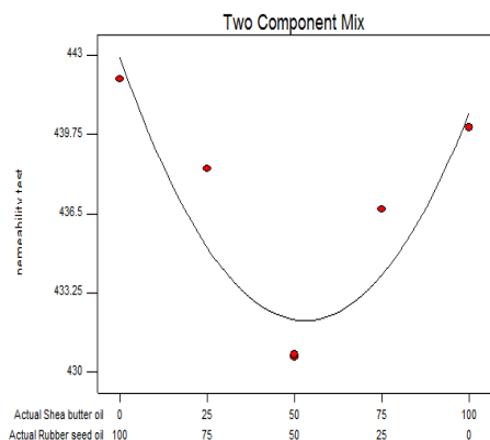
Fig. 38. 0.5% Oil in Sand: Permeability
