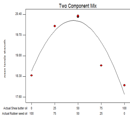
Fig. 26. 0.5% Oil in Sand: Green Tensile Strength
