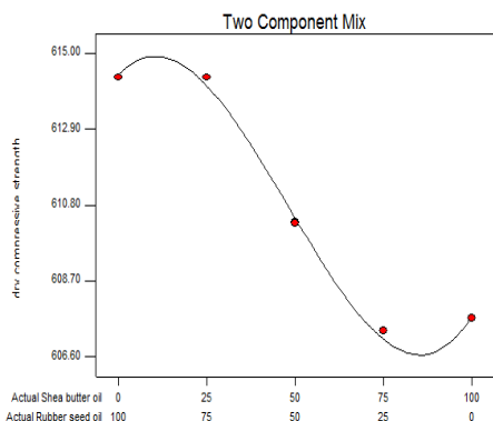
Fig. 24. 2.5% Oil in Sand: Dry Compressive Strength
