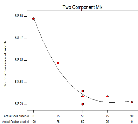
Fig. 22. 1.5% Oil in Sand: Dry Compressive Strength
