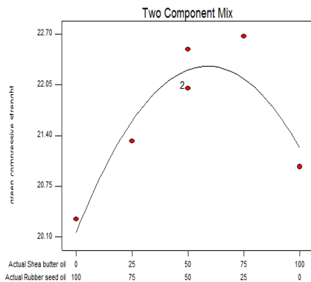
Fig. 14. 0.5% Oil in Sand: Green Compressive Strength
