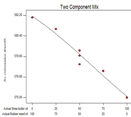
Fig. 21. 1% Oil in Sand: Dry Compressive Strength
