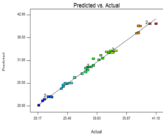
Fig. 8. Predicted vs Actual Response for Green Compressive Strength
