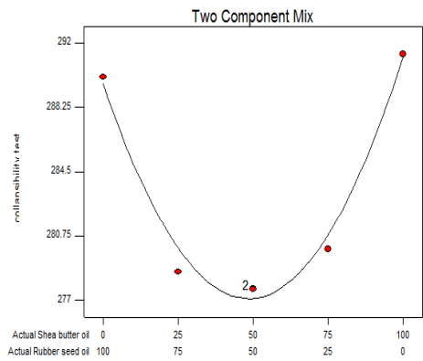
Fig. 44. 0.5% Oil in Sand: Collapsibility
