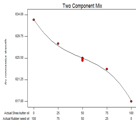
Fig. 25. 3% Oil in Sand: Dry Compressive Strength
