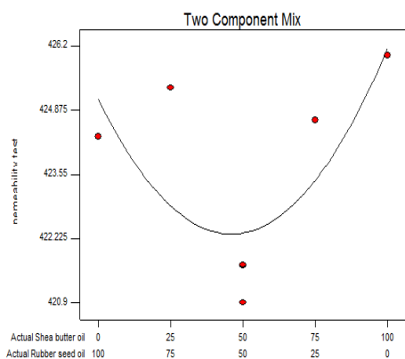
Fig. 41. 2.0% Oil in Sand: Permeability
