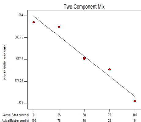
Fig. 36. 2.5% Oil in Sand: Dry Tensile Strength
