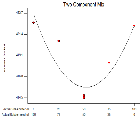
Fig. 42. 2.5% Oil in Sand: Permeability
