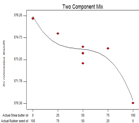
Fig. 20. 0.5% Oil in Sand: Dry Compressive Strength
