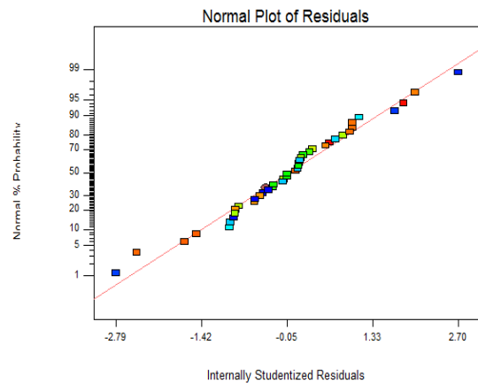
Fig. 7. Normal Plot of Residuals for collapsibility
