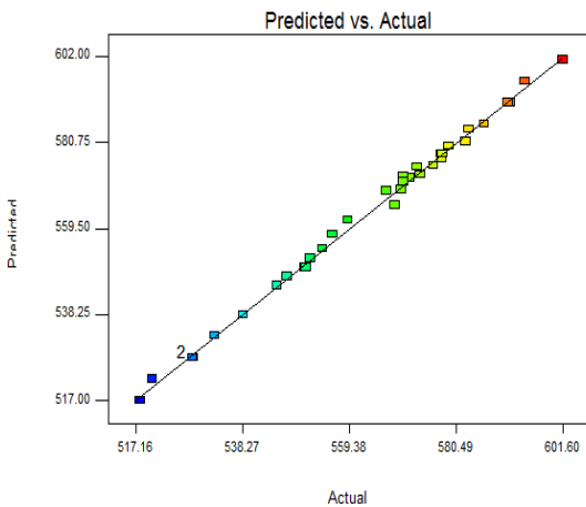
Fig. 12. Predicted vs Actual Response for Dry Tensile Strength
