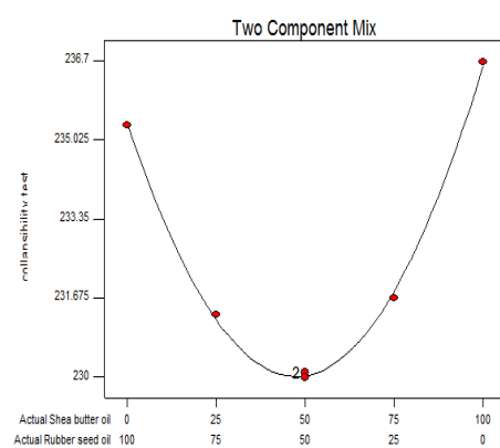
Fig. 47. 2.0% Oil in Sand: Collapsibility
