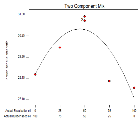
Fig. 29. 2.0% Oil in Sand: Green Tensile Strength
