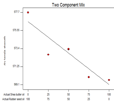
Fig. 35. 2% Oil in Sand: Dry Tensile Strength
