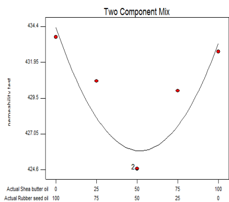
Fig. 40. 1.5% Oil in Sand: Permeability
