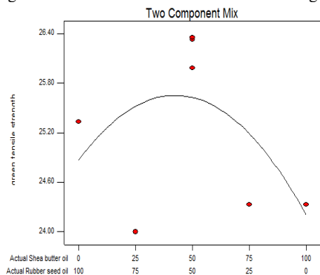
Fig. 28. 1.5% Oil in Sand: Green Tensile Strength
