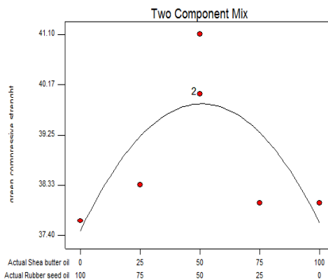
Fig. 19. 3.0% Oil in Sand: Green Compressive Strength
