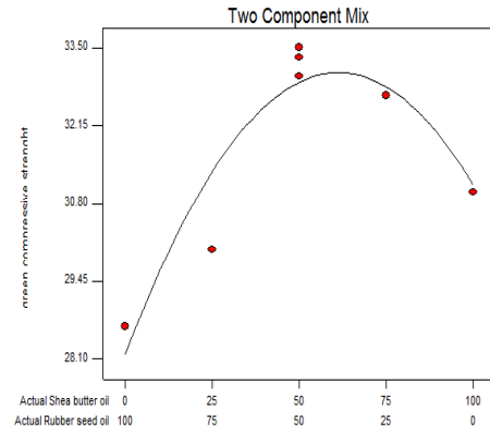
Fig. 17. 2% Oil in Sand: Green Compressive Strength
