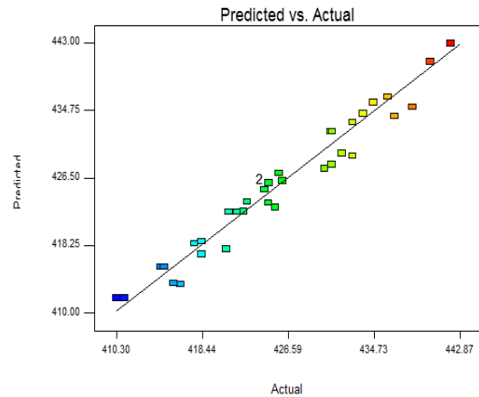
Fig. 3. Predicted vs Actual Response for Permeability
