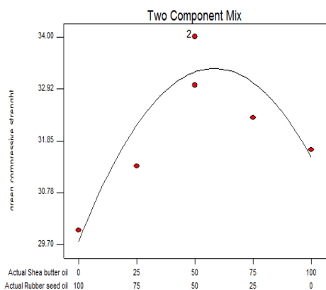
Fig. 18. 2.5% Oil in Sand: Green Compressive Strength
