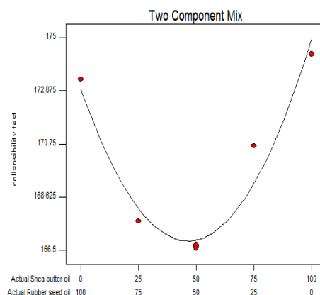
Fig. 49. 3.0% Oil in Sand: Collapsibility
