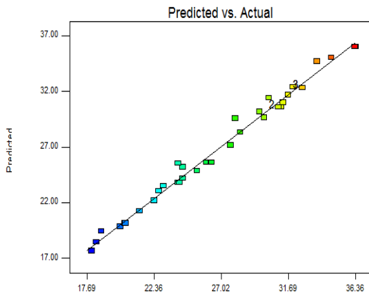
Fig. 10. Predicted vs Actual Response for Green Tensile Strength
