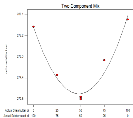
Fig. 45. 1% Oil in Sand: Collapsibility
