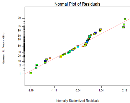
Fig. 2. Normal Plot of Residuals for dry tensile strength
