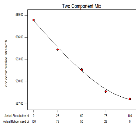
Fig. 23. 2% Oil in Sand: Dry Compressive strength
