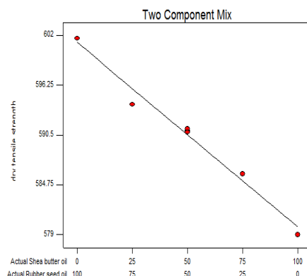
Fig. 37. 3% Oil in Sand: Dry Tensile Strength
