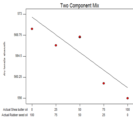
Fig. 34. 1.5% Oil in Sand: Dry Tensile Strength
