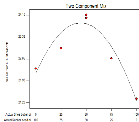
Fig. 27. 1% Oil in Sand: Green Tensile Strength
