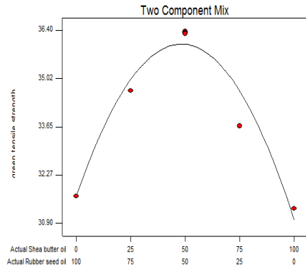
Fig. 31. 3% Oil in Sand: Green Tensile Strength
