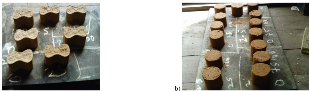
Fig. 1. Moulded Rubber seed – Shea Butter Oil Core Test specimens: (A) Tensile specimens (B) Compression strength, Permeability and collapsibility Test specimens
