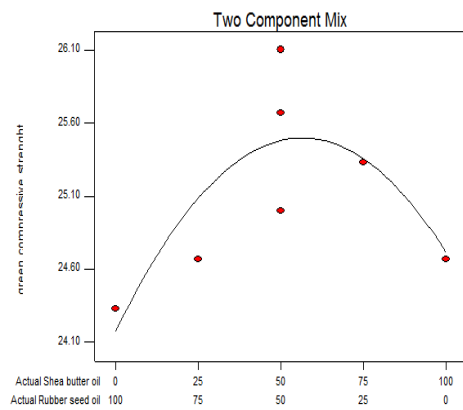
Fig. 15. 1% Oil in Sand: Green Compressive Strength
