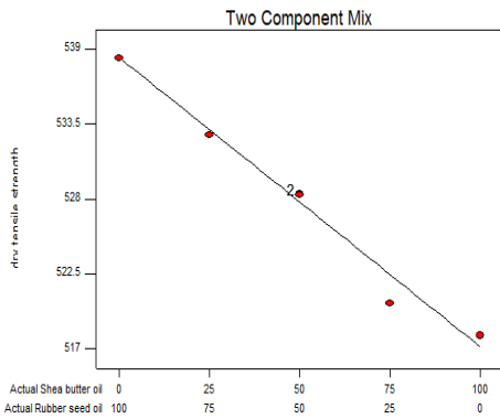
Fig. 32. 0.5% Oil in Sand: Dry Tensile Strength
