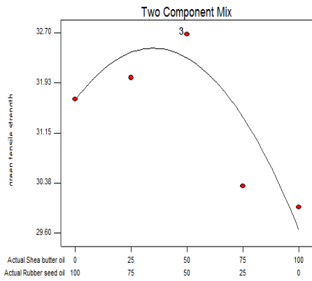
Fig. 30. 2.5% Oil in Sand: Green Tensile Strength
