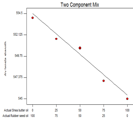
Fig. 33. 1% Oil in Sand: Dry Tensile Strength
