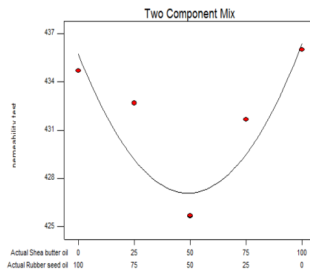
Fig. 39. 1% Oil in Sand: Permeability
