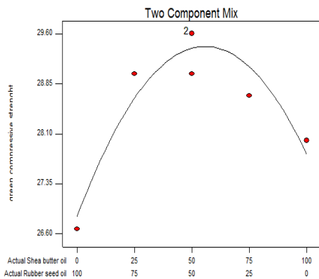
Fig. 16. 1.5% Oil in Sand: Green Compressive Strength
