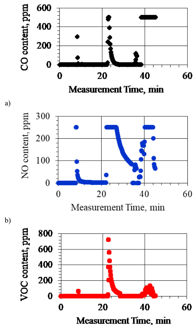
c) Fig. 3. a,b and c are analysis of gases emissions during reduction processes using Carbo-N-Ox reactants
