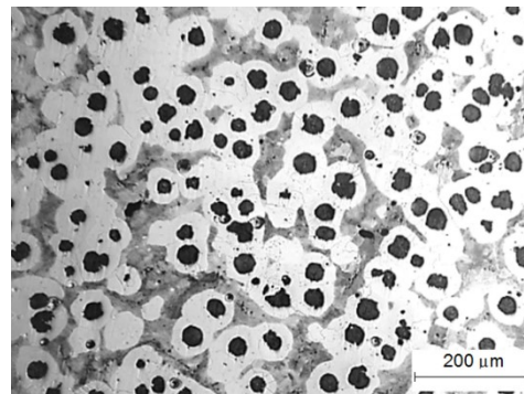
Fig. 2. Microstructure of substrate material. Graphite, ferrite and pearlite. Section etched with Nital. Magnification \times 100
