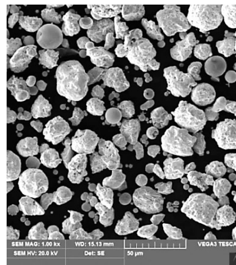
Fig. 3. WCCoCr 86104 powder particles
