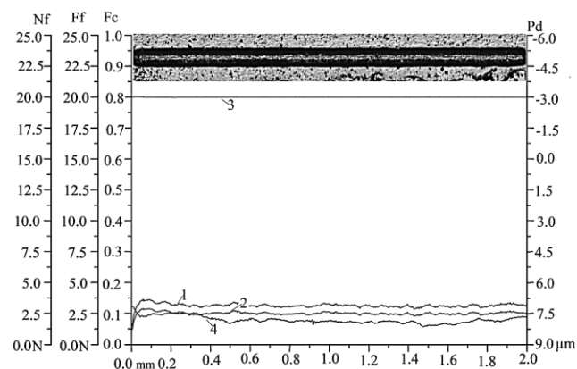
Fig. 5. Scratch test results for WCCoCr coating
