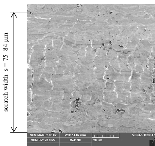
Fig. 6. Scratch test results ductile cast iron
