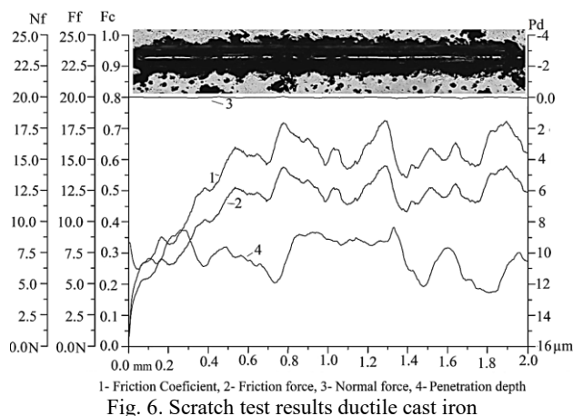
Fig. 6. Scratch test results ductile cast iron
