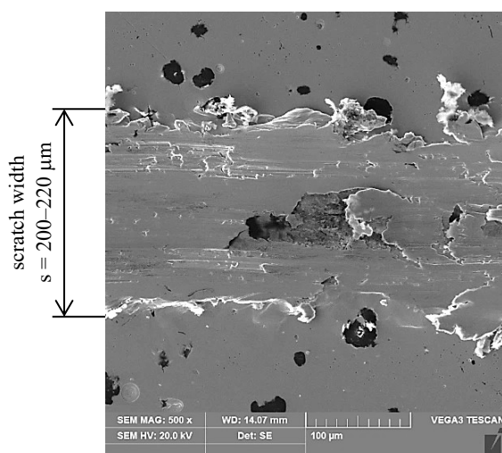
Fig. 7. A view of surface of scratches made on (a) WCCoCr coating and (b) on ductile cast iron substrate. Non-etched sections
