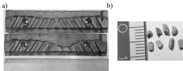
Fig. 1. Excessively worn lining surface (a) resulting in increased percentage share of large-size particle fraction with excessive size (b), unacceptable for the chipboard production process
