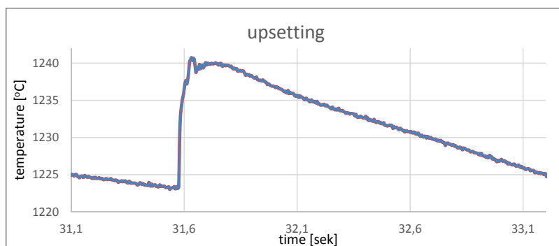
Fig. 3. The temperature of the forging measured in its axis during the upsetting process
