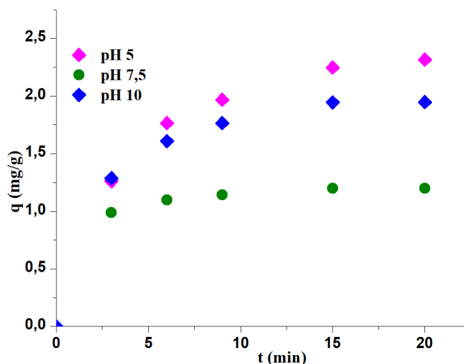
Fig. 4. Effect of solution pH and contact time on tannic acid adsorption onto fluorite
