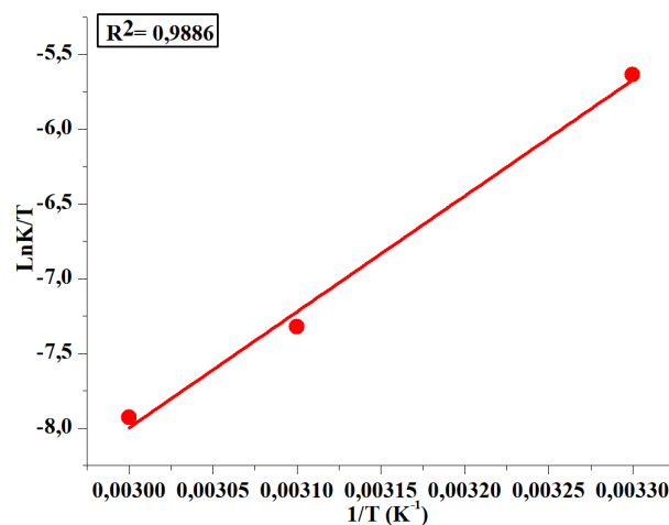
Fig. 6. Graphical representation of the variation of ln k/T versus 1/T for tannic acid adsorption onto fluorite
