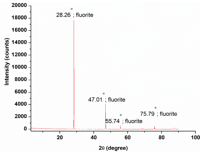
Fig. 1. XRD spectra of fluorite mineral
