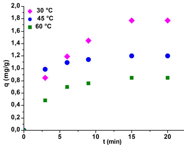
Fig. 5. Effect of temperature and contact time on tannic acid adsorption onto fluorite
