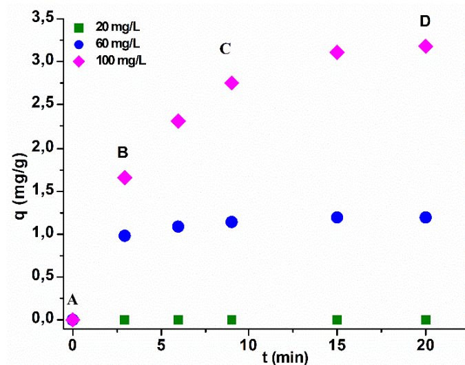
Fig. 3. Effect of initial tannic acid concentration and contact time on tannic acid adsorption onto fluorite
