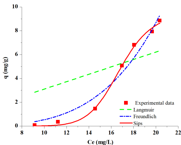
Fig. 2. Non-linear fitting of tannic acid adsorption onto fluorite
