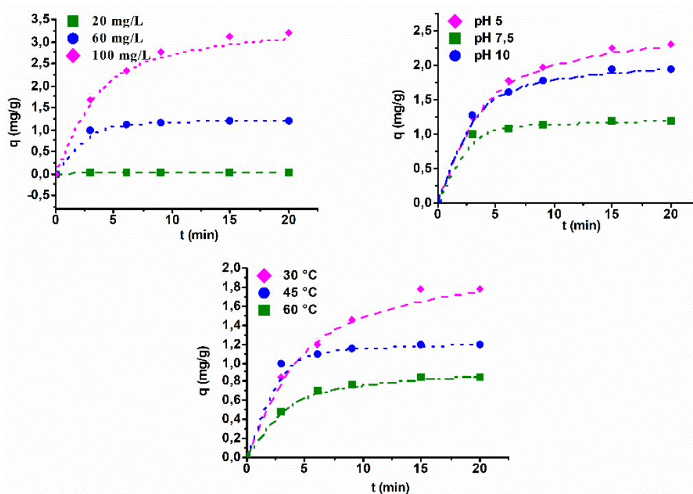
Fig. 6. Pseudo n order kinetic model of tannic acid adsorption onto fluorite at various initial tannic acid concentrations, solution pH and temperature
