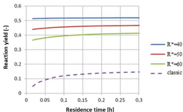
Figure 7. Reaction yield as a function of residence time, in a classical reactor and in membrane reactor at different value of R^* (60°C, pH 7.0, thermolysin concentration 0.005 g/L, bovine serum albumin concentration 2 g/L)
