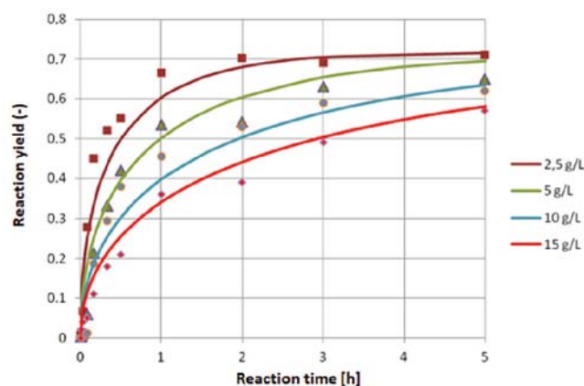
Figure 4. Dependence of the reaction yield from reaction time for the albumin-pepsin system (37°C, pH 2.0, enzyme concentration 0.005 g/L, bovine serum albumin 2.5–15 g/L); points – experimental data; lines – model calculations
