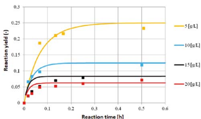
Figure 3. Dependence of the reaction yield from reaction time for the albumin-thermolysin system (60°C, pH 7.0, enzyme concentration 0.005 g/L, bovine serum albumin 5–20 g/L); points – experimental data; lines – model calculations
