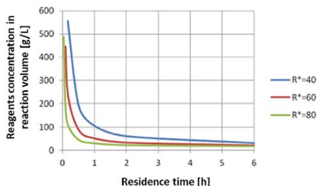
Figure 6. Influence of membrane selectivity ( R^* = 40\text{--}80 ) on reagents concentration in reaction volume at different residence times
