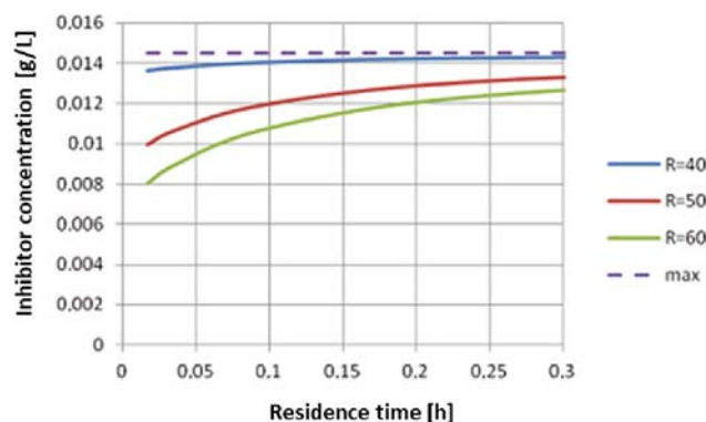
Figure 8. Inhibitor concentrations as a function of residence time in a membrane reactor at different value of R^* (60°C, pH 7.0, thermolysin concentration 0.005 g/L, bovine serum albumin concentration 2 g/L)
