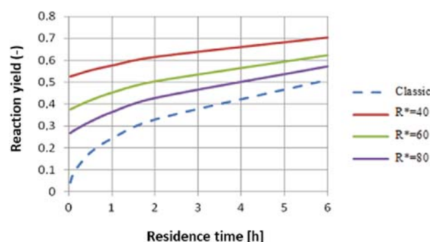
Figure 5. Reaction yield as a function of residence time, in a classical reactor and in a membrane reactor at different value of R^* (50°C, pH 7.0, subtilisin concentration 0.01 g/L, bovine serum albumin concentration 15 g/L)
