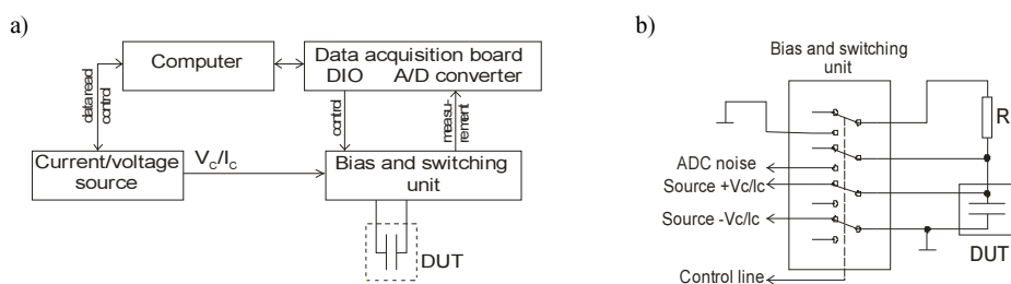
Fig. 4. The measurement setup: a block diagram (a); a switching and biasing unit (b).
