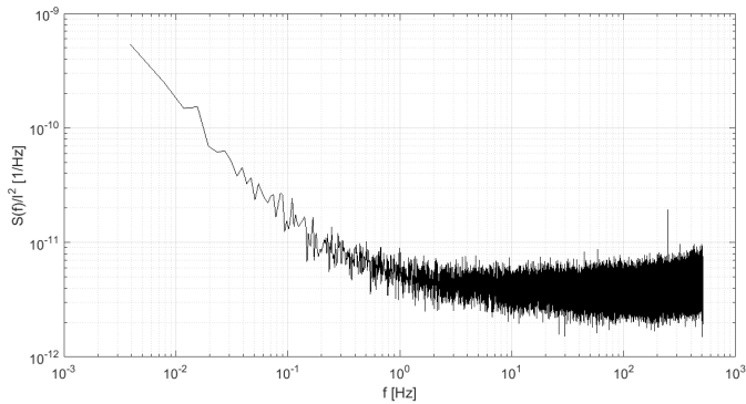
Fig. 7. Power spectral density of current fluctuations S(f) identified in the discharging current I of a DRL 2.7V 10F specimen when discharged through the loading resistance 1 k \Omega . Power spectrum estimated in each time interval was normalized by the square of the discharging current.
