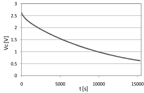
Fig. 5. A discharging curve of the tested supercapacitor, DRL 2.7V 10F type, through the loading resistance of 1 k \Omega .
