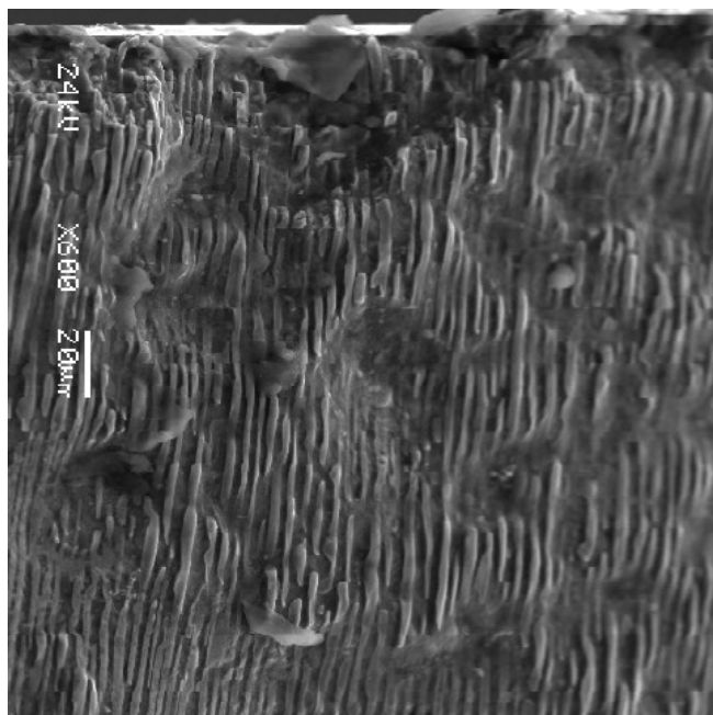
Fig. 3. Fracture surfaces of directionally solidified Fe-4,25%C composites with average lamellar spacing of 8,25 µm, SEM
