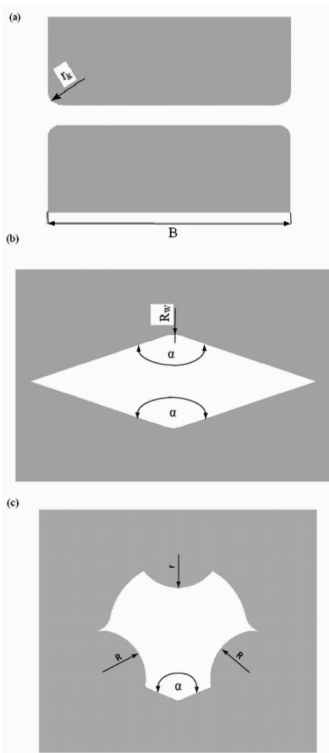
Fig. 2. Shape of anvils: (a) – flat ( r_k = 0.10B ), (b) – radial-rhombic with an impression angle of \alpha = 135^\circ/135^\circ ( R_w = 0.35D_0 ), (c) – special tri-radial ( R/D_0 = 0.40 , r/D_0 = 0.35 and \alpha = 135^\circ )
