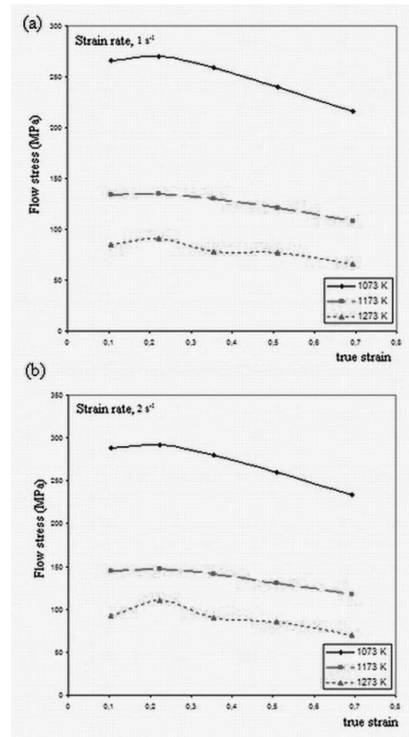
Fig. 1. Variation of flow stress for the Ti-6Al-4V alloy as a function of true plastic strain and temperature, for different strain rate values, i.e.: (a) – \dot{\epsilon} = 1s^{-1} and (b) – \dot{\epsilon} = 2s^{-1}
