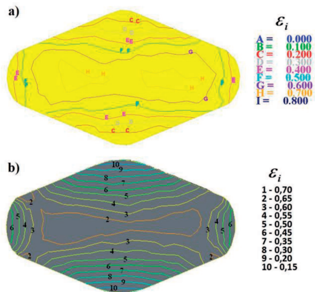
Fig. 9. Comparison of the theoretical (a) and experimental (b) effective strain ( \varepsilon_i ) distribution on the cross-sectional surfaces of Ti-6Al-4V alloy specimens deformed in radial-rhombic anvils with an impression angle of \alpha = 135^\circ/135^\circ . Relative feed l_w = 0.75 , true strain \varepsilon_h = 0.35
