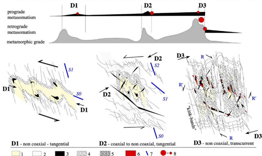
Fig. 4. Conceptual model for the generation of Mg - Al - B - calcsilicate gemstones – dependent on fluid / rock interaction in the presence of tangential to transcurrent shear deformation. 1 - calc - magnesium siliceous metacarbonate rock; 2 - magnesian calcsilicate rock; 3 - dilatational environments, occasionally miarolitic; 4 - masses of deformed inosilicates and phyllosilicates with newly formed blasts; 5 - cataclasis and mylonite; 6 - deposition sites for noble minerals; 7 - metamorphic surfaces; 8 - probable chronological position for the genesis of gemstones, with the relative importance, qualitatively indicated by the diameter of the representative circle.
