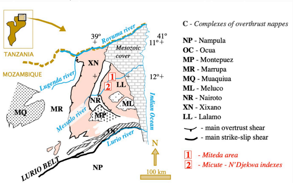
Fig. 1. Paleogeographic and tectonic organization of the Cabo Delgado Proterozoic terranes (modified from [6] and [7]) – Location of the main gem-deposits considered in the present study – Miteda (1) and Micute-N'Djekwa (2).
