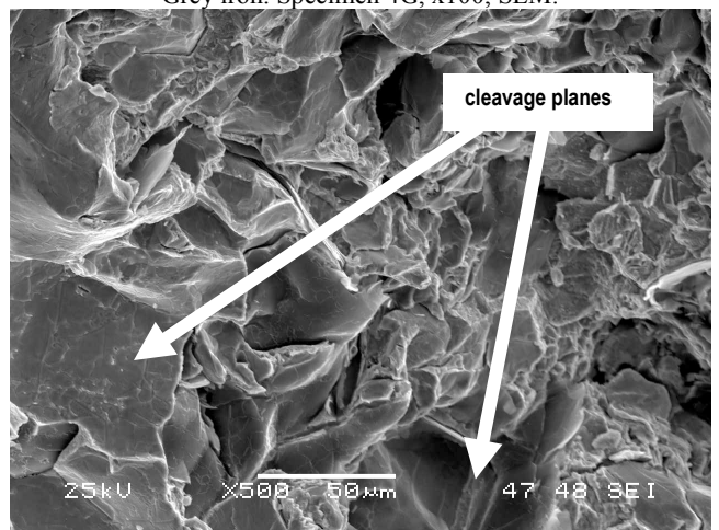
Grey iron. Specimen 4G, x500, SEM.
