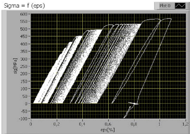
Fig. 2. The stress-strain diagram obtained during specimen cycling according to MLCF methodology. EN-GJS-600-3
