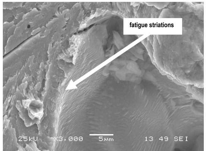
Ductile iron. Specimen 3, x3000, SEM.
