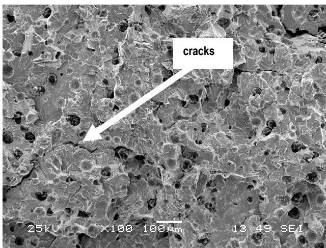
Ductile iron. Specimen 3, x100, SEM.
