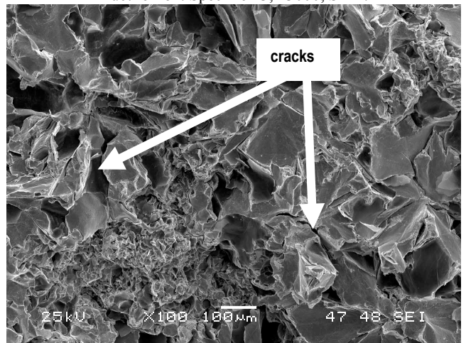
Grey iron. Specimen 4G, x100, SEM.
