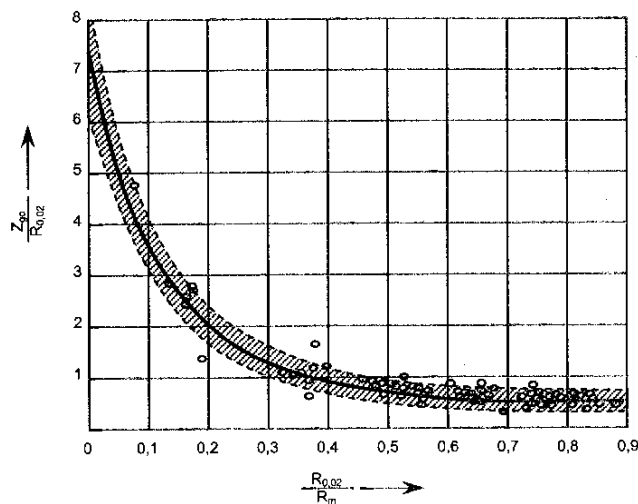
Fig. 1. Curve used in fatigue strength assessment [15]
