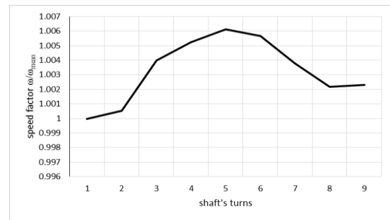
Fig. 7. Mean values of speed factor referring to subsequent shaft revolutions recorded during sea waving (9 revolutions)
