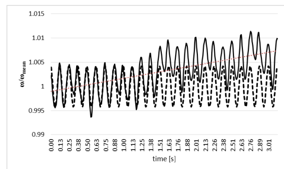
Fig. 4. Comparison of modelled function of speed factor (dotted line) and function of speed factor recorded on real object at waving sea (solid line)
