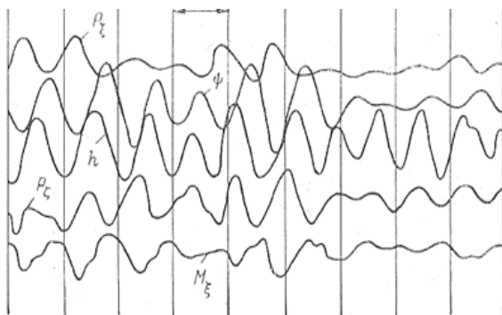
Fig. 1. Model – based courses of: propeller's draught – h , revolutionary torque – M_{\xi} , thrust – P_{\xi} and vertical force – P_{\zeta} as result of hull's pitch angle \psi [2]
