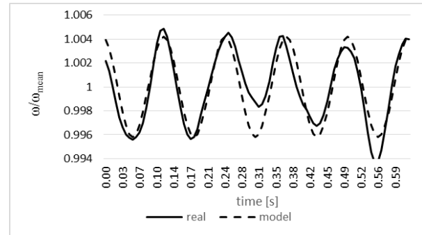
Fig. 3. Comparison of recorded run of speed factor (solid line) and model one (dotted line)
