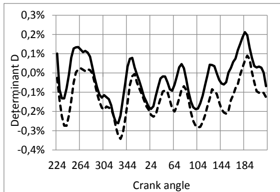
Fig. 10. Comparison of determinant D of healthy engine obtained from data collected without waving impact (dotted line) and with waving (solid line)
