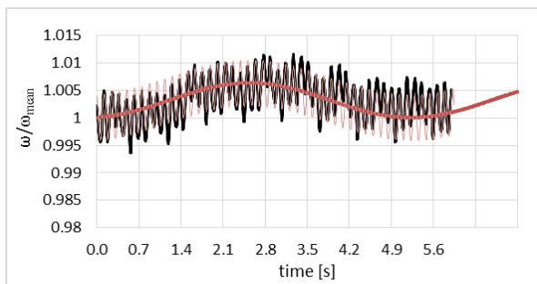
Fig. 5. Speed factor course as superposition of pistons contribution and sea waving.
