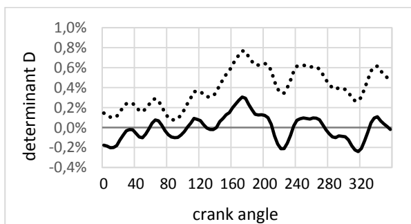
Fig. 6. comparison of determinant D for healthy engine working at calm sea (solid line) and rough sea (dotted line)
