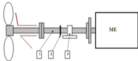
Fig. 2. Scheme of ship's shafting arrangement
