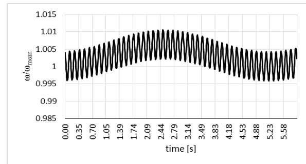
Fig. 8. Model course of speed factor of an engine working at wavering sea
