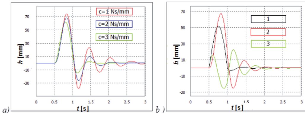
Fig. 7. The dynamic answer of the assembly to the unit excitation for the case of the rim made of AlSi: displacement of car body vs. time for different values of damping coefficient (a), and displacement of car body vs. time for the damping coefficient c = 1.8 (b): 1 – displacement of the wheel, 2 – displacement of the car body, 3 – displacement of the rod of shock absorber
