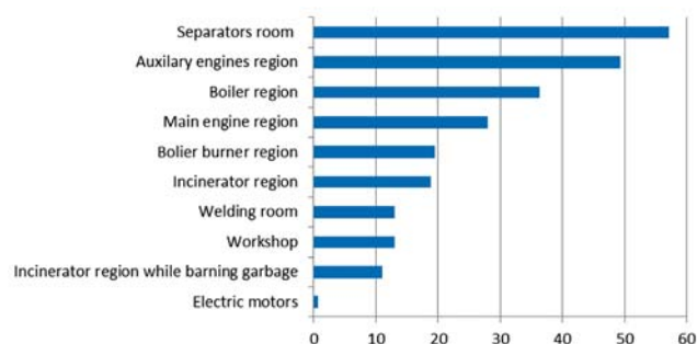
Fig. 4. Places requiring special supervision in the engine room as a percentage of respondents
