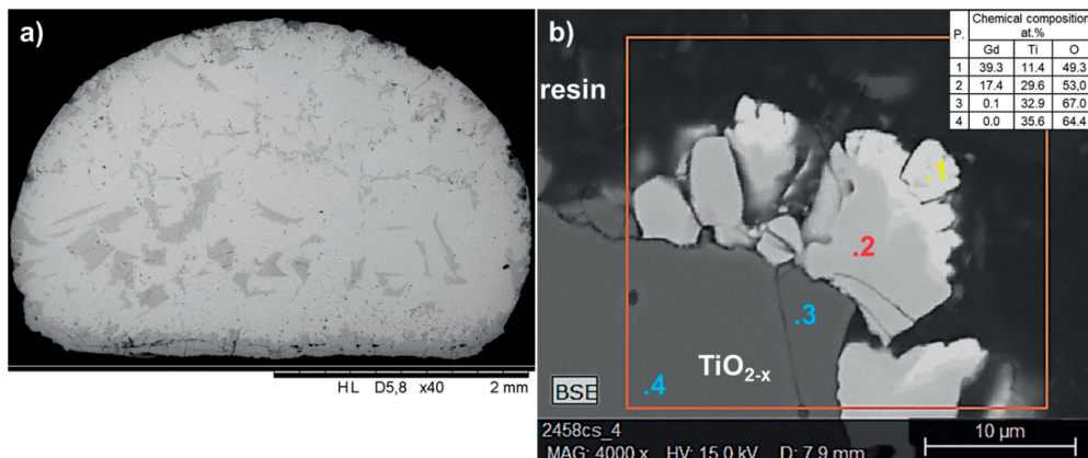
Fig. 5. a) SEM image of the detached Gd drop of the Gd/ \text{TiO}_2 couple, b) SEM/EDS analysis of the substrate-side interface of the Gd/ \text{TiO}_2 couple performed on the substrate in situ detached after the wettability test
