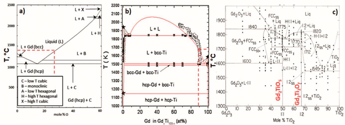
Fig. 6. Phase diagram data: a) Gd-O [12], b) Gd-Ti [13], c) Gd 2 O 3 -TiO 2 [14]
