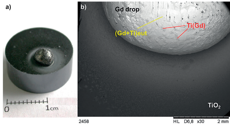
Fig. 2. The Gd/TiO 2 couple after wettability tests: a) photo, b) SEM top-view image
