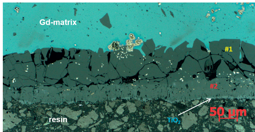
Fig. 4. Structure of the Gd/ \text{TiO}_2 interface from the drop side after the wettability tests (OM)
