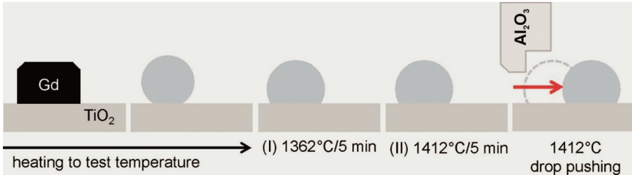
Fig. 1. Sessile drop method combined with classical contact heating and the drop pushing procedure used during the wettability tests
