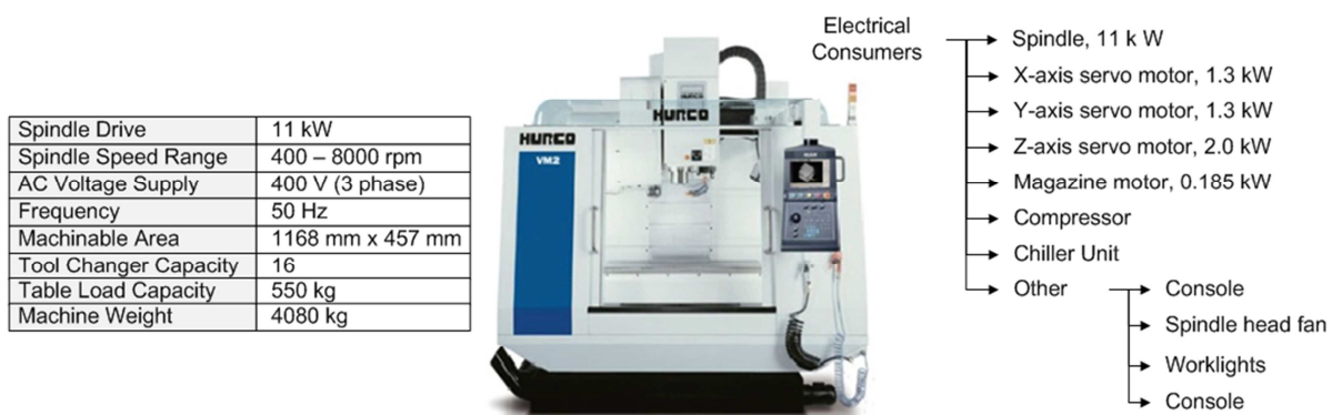
Fig. 5. Hurco 3-Axis CNC machine tool overview
