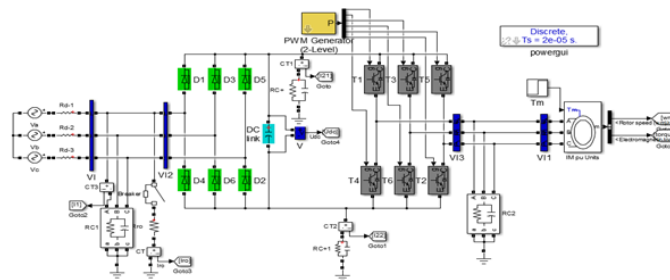
Fig. 7. Simulation model of mine power transmission network DC
