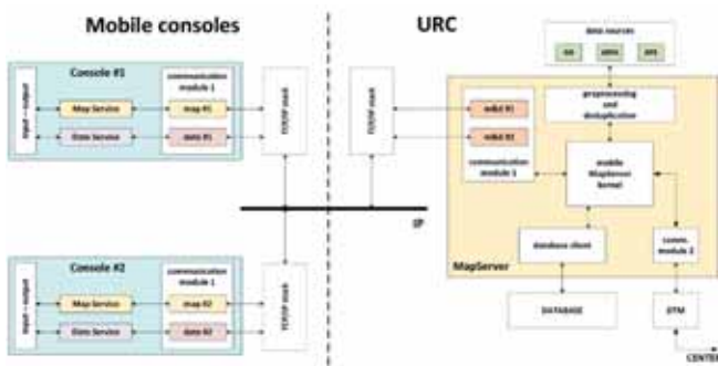
Fig. 4. A block diagram illustrating the major functional modules of mobile MapServer and consoles
