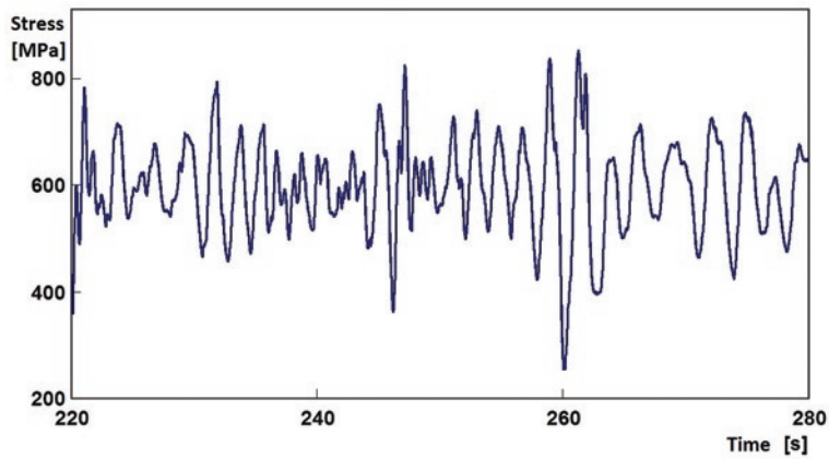
Fig. 6. Example of the stress pattern of a leaf spring installed on the rear axle of a vehicle (values do not include preliminary stresses due to peening)
