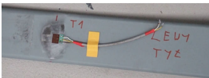
Fig. 4. Leaf spring with glued-on strain gauge
