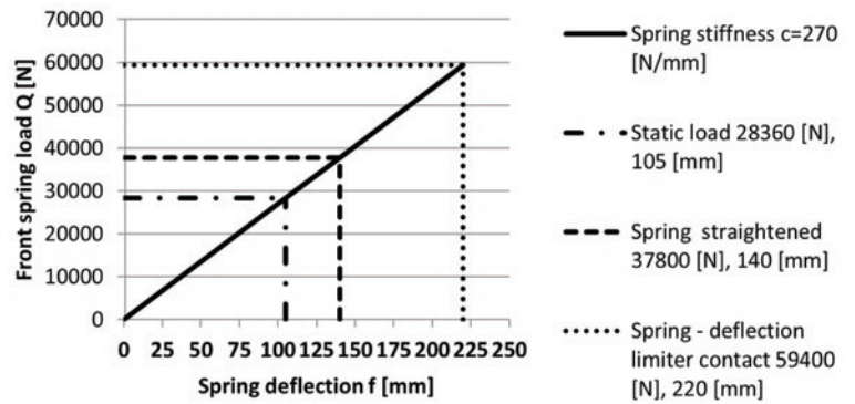
Fig. 1. Stiffness characteristics of the front axle parabolic spring
