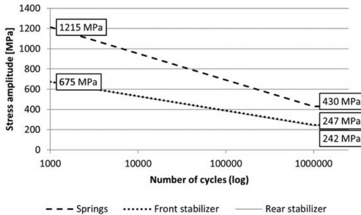
Fig. 3. Determined diagrams of fatigue strength of springs and stabilizers
