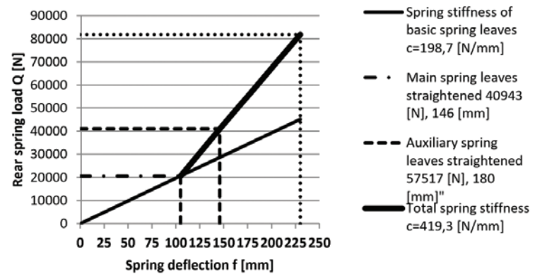
Fig. 2. Stiffness characteristics of the rear axle parabolic spring
