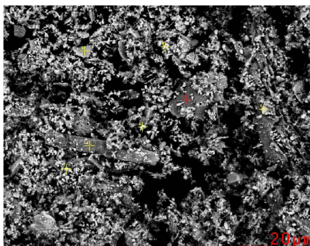
Fig. 3. SEM image of fly ash and point (red +) to XRF analysis
