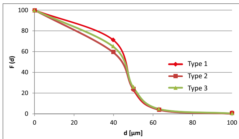
Fig. 1. Grain composition of tested samples of fly ashes Type 1 – obtained from a batch containing 20% agromass in the form of straw, Type 2 – 20% in the form of dried fruit, Type 3 – 20% in the form of slates of palm nut
