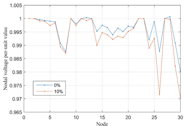
Fig. 7. Nodal voltage per-unit values when EV permeability equals 10%
