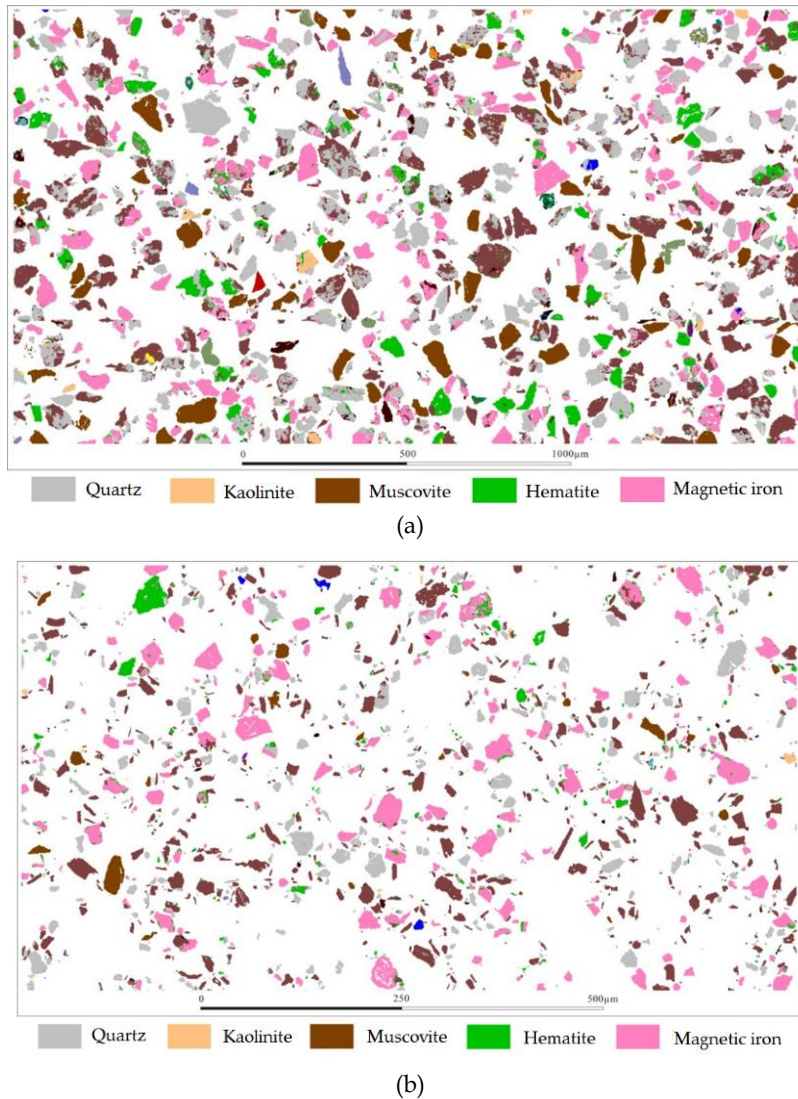
Fig. 11. The mineral map of the roasted products. (a) the particle size of -38 \sim +75 \mu\text{m} and (b) particle size of -38 \mu\text{m}
