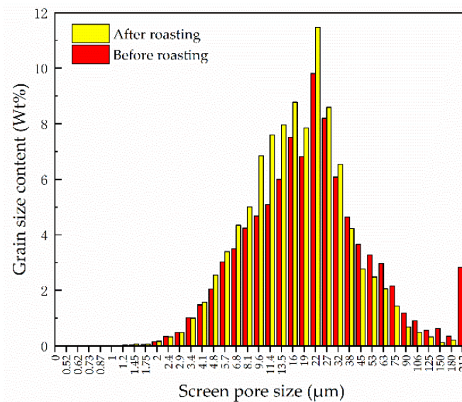
Fig. 8. The particle size distribution of siderite in the LGRIT before and after roasting
