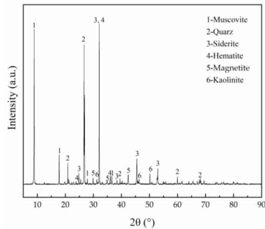
Fig. 2. The results of XRD diffraction analysis of the LGRIT
