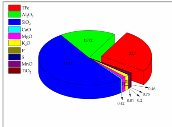
Fig. 6. The results of chemical multi-element analysis of the roasted products
