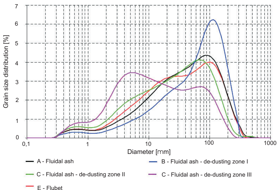
Fig. 1. Distribution of grain size of fly ash used in analyses – differential curves (Małolepszy, 2010)
