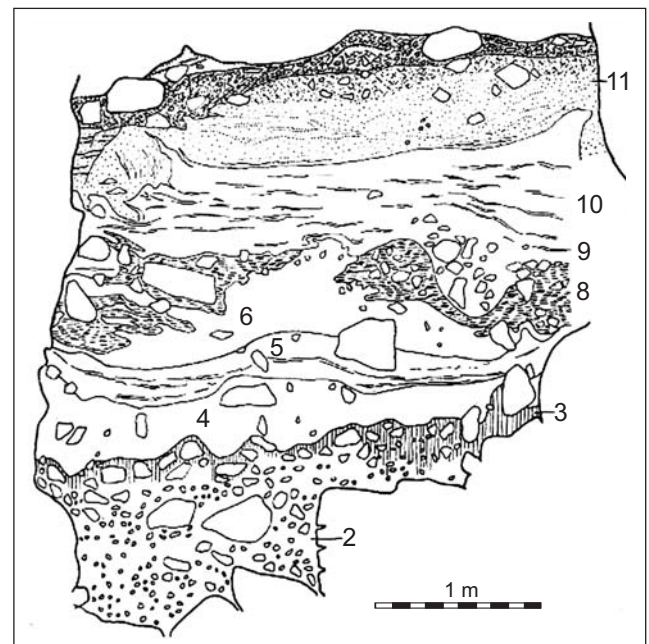
Fig. 3. Schematic transversal cross-section of sediments in the Korytarz Wstępny (Entrance Passage) of Raj cave (based on materials of J.K. Kozłowski, simplified); copy from the publication of Madeyska (1974) – numbers of lithological units were corrected (lack of units 7 and probably 12 in this cross-section).
