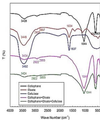
Fig. 5. FTIR spectra of collophane, oleate, cellulase and treated collophane
