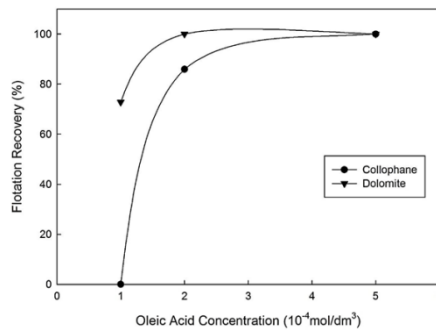
Fig. 1. Effect of oleate concentration on floatability of collophane and dolomite single minerals
