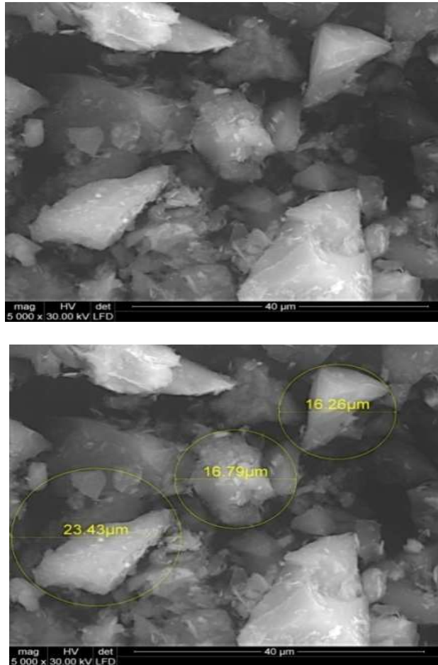
Fig. 2. General view of comminuted coal particles
