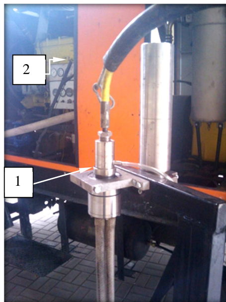
Fig. 1. General view of hydrojetting comminution apparatus prototype (1 - hydrojetting grinder, 2 – HDP 164 type hydro-monitor)
