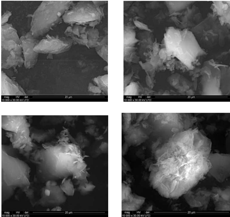
Fig. 5. SEM pictures of hard coal showing different stage of their specific surface development
