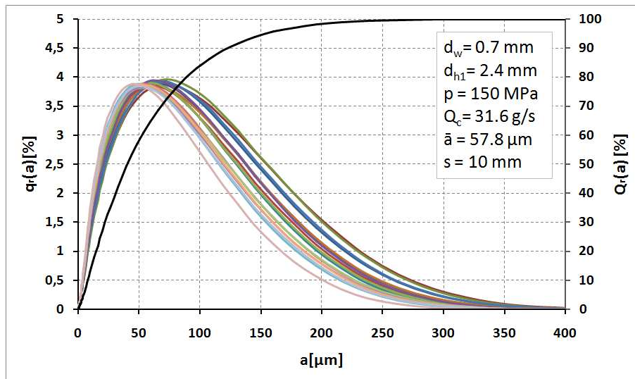
Fig. 3. Distributions of hard coal particles fraction comminuted with water pressure of 150MPa
