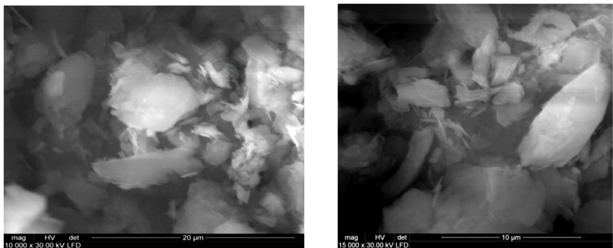
Fig. 9. SEM pictures of brown coal comminuted with high-pressure water jet of 250MPa showing different stage of their specific surface development
