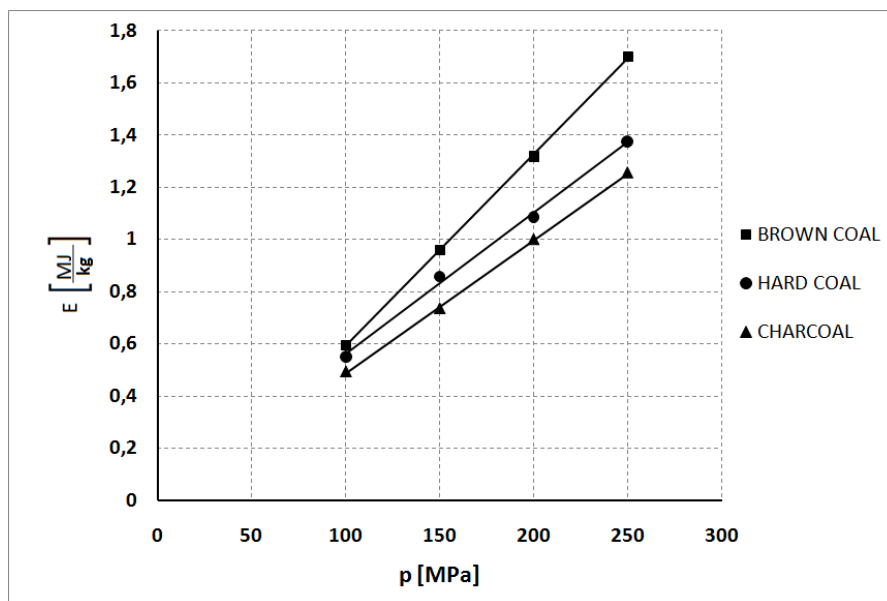
Fig. 15. Dependence of unitary energy consumption E indispensable for processing of 1 kg of different coal types vs. nominal water jet pressure ( d_w = 0,7\text{mm} ; d_h = 2,4\text{mm} )
