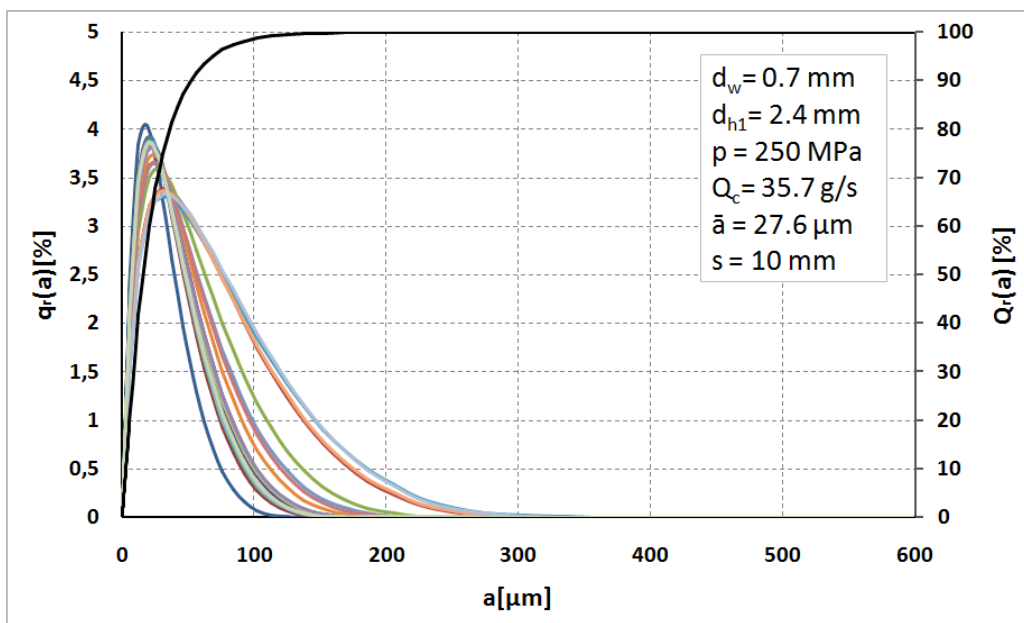
Fig. 7. Distributions of brown coal particles fraction comminuted with water pressure of 250MPa
