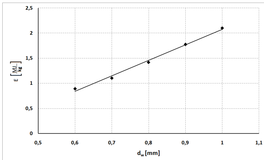
Fig. 14. Dependence of unitary energy consumption E indispensable for processing of 1 kg of hard coal vs. water nozzle diameter d_w ( p = 200\text{MPa} , d_h = 2,4\text{mm} )
