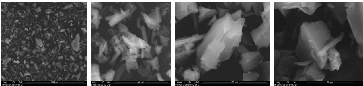
Fig. 13. SEM pictures of charcoal showing different stage of their specific surface development
