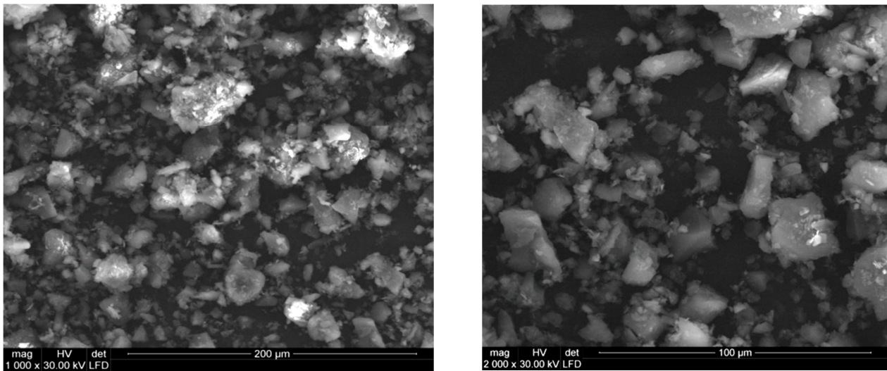
Fig. 8. SEM images illustrating diversification of brown coal size and shape after high-pressure water jet comminution (p= 250MPa)
