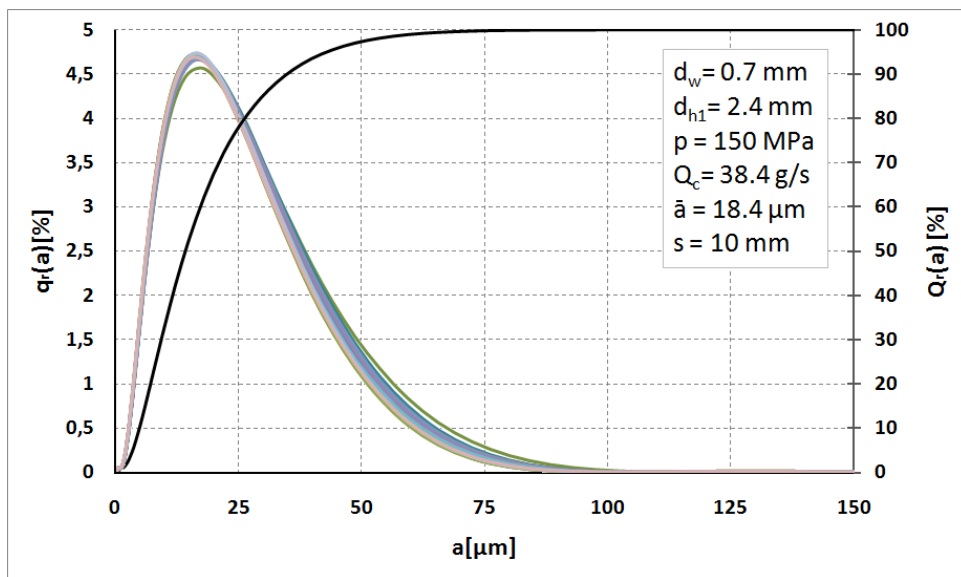
Fig. 10. Distributions of charcoal grains fractions comminuted with water pressure of 150MPa
