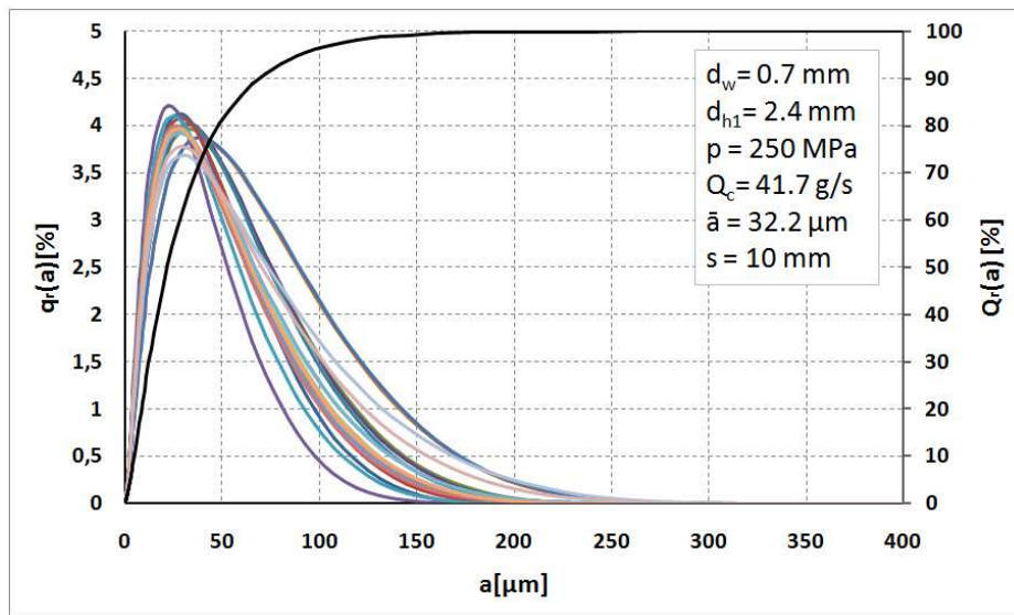
Fig. 4. Distributions of hard coal particles fraction comminuted with water pressure of 250MPa
