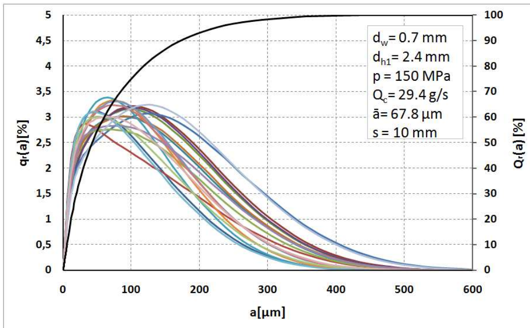
Fig. 6. Distributions of brown coal particles fraction comminuted with water pressure of 150MPa
