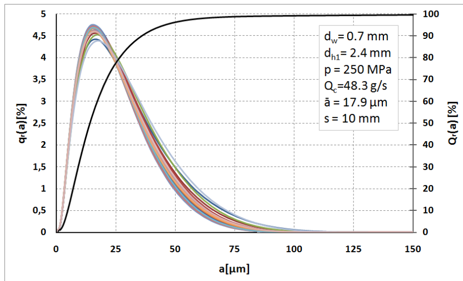
Fig. 11. Distributions of charcoal grains fractions comminuted with water pressure of 250MPa
