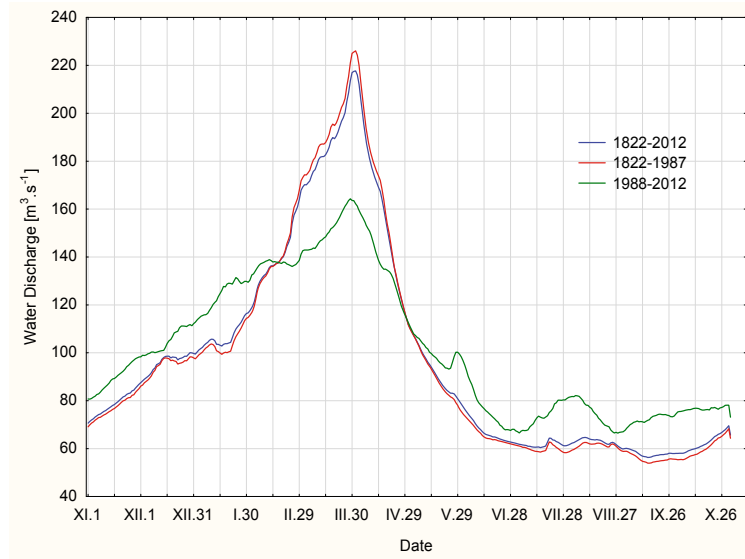
Fig. 5. Averaged daily water discharges of the Warta River in Poznan in periods of 1822–2012, 1822–1987 and 1988–2012
