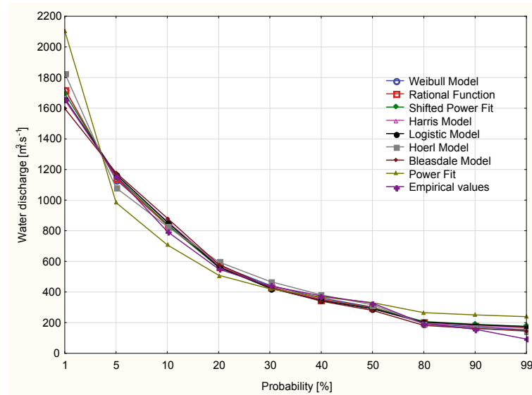
Fig. 8. Estimation of probability values of maximum yearly empirical water discharges (Empirical values) together with higher discharges by selected models; for the Warta River in Poznan
