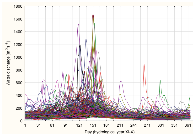
Fig. 1. Daily water discharges of Warta River in the Poznan cross-section in 1822–2012
