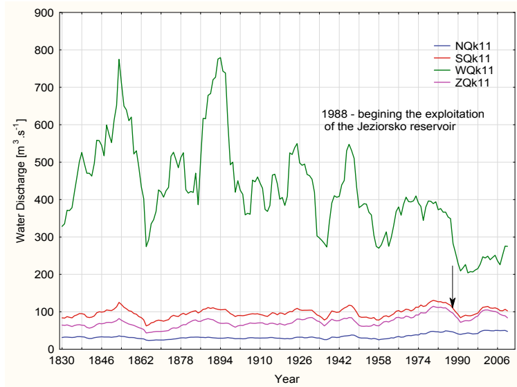
Fig. 2. 11-year smoothed means of first degree characteristic water discharges of the Warta River in Poznan
