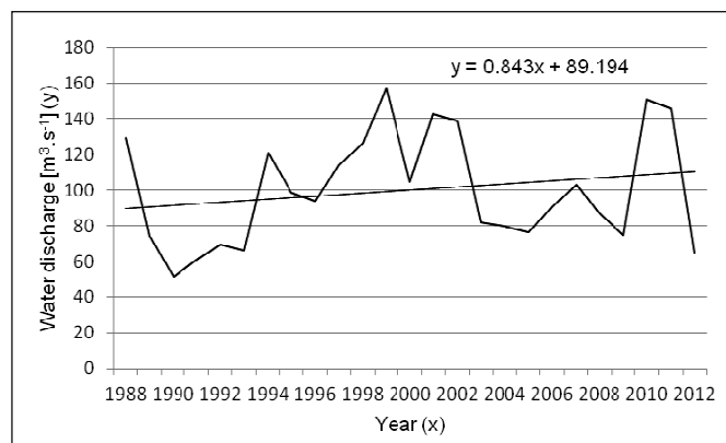
Fig. 6. Mean yearly water discharges of the Warta River in Poznan in periods 1822–2012, 1822–1987 and 1988–2012
