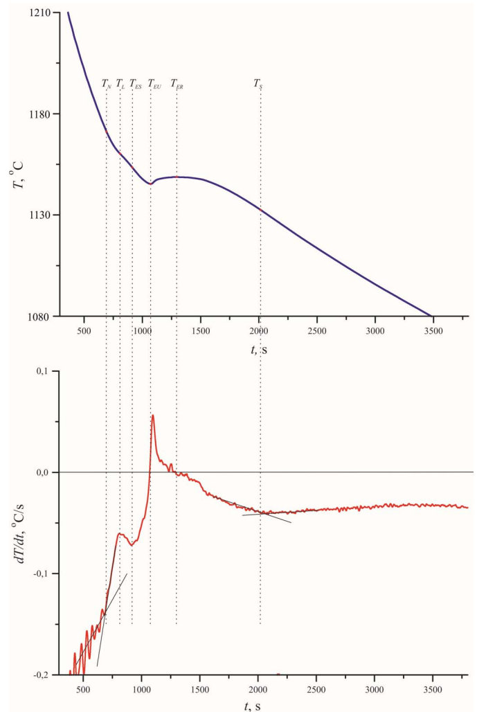
Fig. 4. Cooling curve recorded on the cone block and its first derivative
