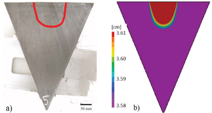
Fig. 6. Cross-section of the cone block and thermal modulus (cm)
