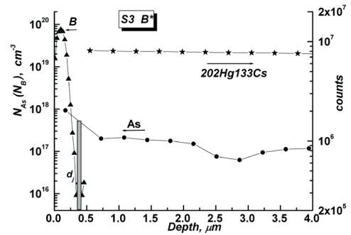
Fig. 9. SIMS distribution of As and signal of the main component of \text{CdXHg}_{1-x}\text{Te} solid solution (Hg concentration) in near-surface regions for epitaxial structure of sample S3 B*
