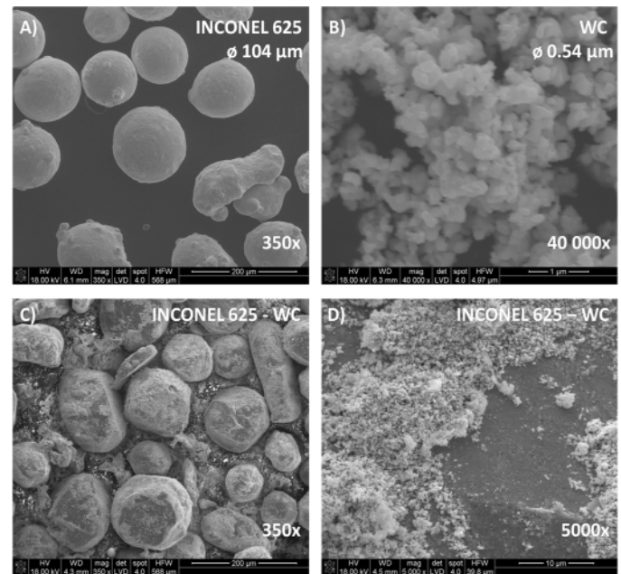
Fig. 2. SEM images showing: A – Inconel 625 powder; B – WC powder; C, D – Inconel 625 – WC mixture after 90 minutes of homogenisation
