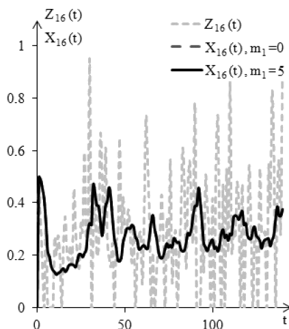
Fig. 12. Obtained values X_{16}(t) and the desired values Z_{16}(t) during learning with using gradient method type (3), (5)
