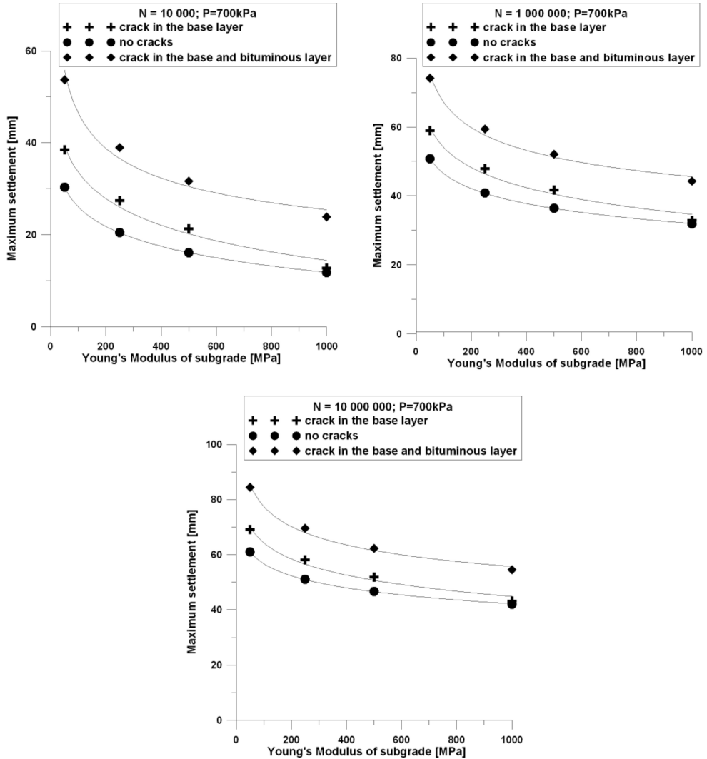
Fig. 7a. Variation in maximum pavement settlements with the subgrade modulus. Comparison of pavement behaviour during three phases of deterioration: P = 700 kPa. Load applied asymmetrically with regard to the crack.
