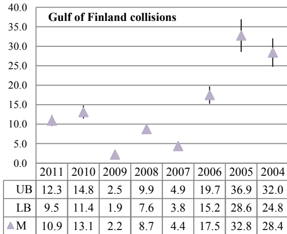
Figure 13. Estimate for true number of Gulf of Finland collisions
