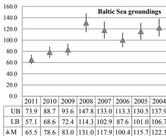
Figure 12. Estimate for true number of Baltic Sea groundings
