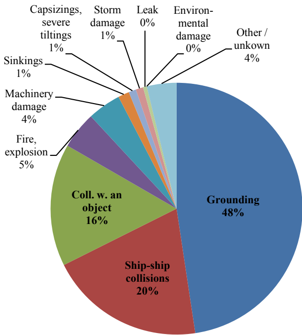
Figure 5. Accidents in the GoF according to DAMA and HELCOM databases 1997–1999 and 2001–June 2006 (Kujala et al., 2009)
