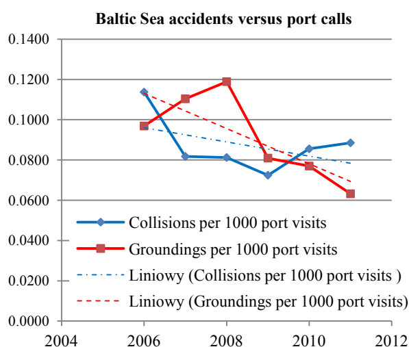
Figure 9. Accidents per 1000 port visits or line crossings in the Baltic Sea along with linear trend lines
