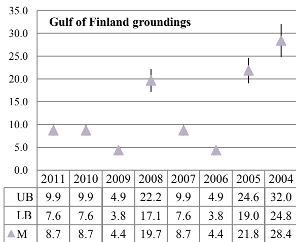
Figure 14. Estimate for true number of Gulf of Finland groundings
