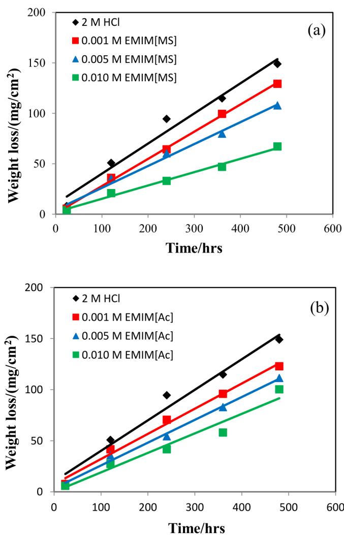
Fig. 2. Variation of weight loss ( \text{mg/cm}^2 ) with time (hrs) for the corrosion of carbon steel in 2 M HCl containing various concentrations of (a) EMIM[MS] and (b) EMIM[Ac]
