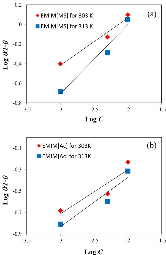
Fig. 6. El-Awardy kinetic-thermodynamic model for the adsorption of (a) EMIM[MS] and (b) EMIM[Ac] on API 5L X52 carbon steel at 303 K and 313 K
