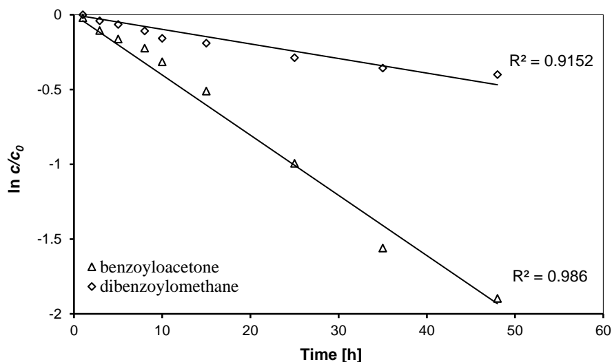
Fig. 2. Kinetics of Cu(II) ions transport across PIMs containing 0.05 M benzoyloacetone (1) and dibenzoyl methane (2) from aqueous solutions. Feed phase: c_M = 1 mM, pH = 7.8, receiving phase: 0.5 M HCl, Membrane: 0.5 g PVC, 0.2 g ADO, and 60% carrier calculated on PVC
