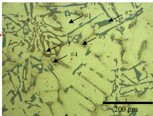
Fig. 2. Derivative curie, cooling curve, baseline as well the related microstructure for the cylindrical sample cooled with a cooling rate of 0,2°C/s, 1 - \alpha , 2 - \beta , 3 - \text{Al}_{12}(\text{FeMn})_3\text{Si} , 4 - \text{Al}_2\text{Cu} , 5 - \text{Mg}_2\text{Si}
