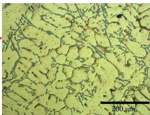
Fig. 2. Derivative curie, cooling curve, baseline as well the related microstructure for the cylindrical sample cooled with a cooling rate of 0,2°C/s, 1 - \alpha , 2 - \beta , 3 - \text{Al}_{12}(\text{FeMn})_3\text{Si} , 4 - \text{Al}_2\text{Cu} , 5 - \text{Mg}_2\text{Si}
