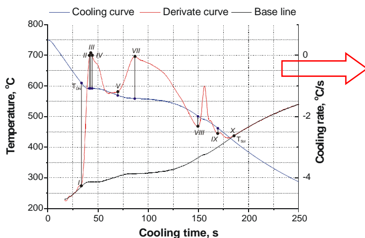
Fig. 3. Derivative curie, cooling curve, baseline as well the related microstructure for the cylindrical sample cooled with a cooling rate of 1,0°C/s
