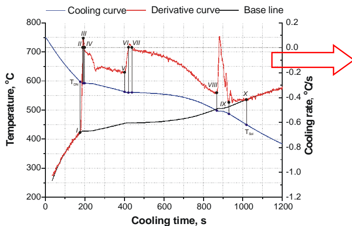
Fig. 2. Derivative curie, cooling curve, baseline as well the related microstructure for the cylindrical sample cooled with a cooling rate of 0,2°C/s, 1 - \alpha , 2 - \beta , 3 - \text{Al}_{12}(\text{FeMn})_3\text{Si} , 4 - \text{Al}_2\text{Cu} , 5 - \text{Mg}_2\text{Si}
