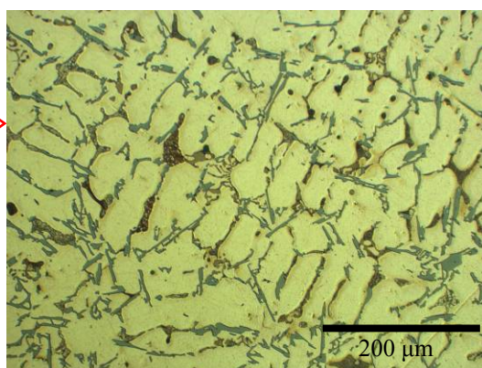
Fig. 3. Derivative curie, cooling curve, baseline as well the related microstructure for the cylindrical sample cooled with a cooling rate of 1,0°C/s
