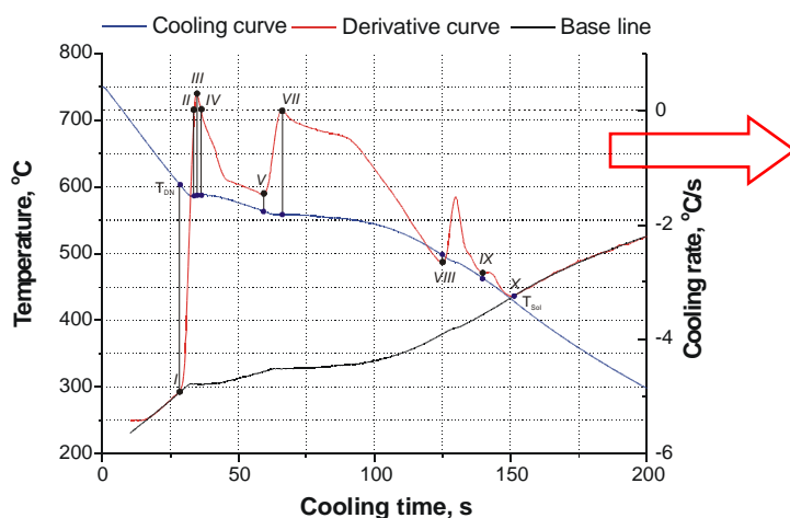
Fig. 4. Derivative curie, cooling curve, baseline as well the related microstructure for the cylindrical sample cooled with a cooling rate of 1,25°C/s
