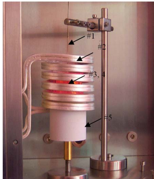
Fig. 1. Scheme of the heating and cooling system of the UMSA device as well the placement of the thermoelements: 1 – thermocouple, 2 – heating coil – cooling nozzles, 3 – steal foil, 4 – sample, 5 – sampler isolation
