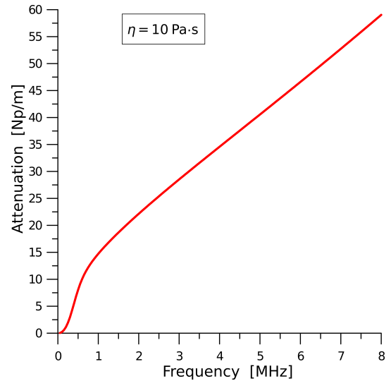
Fig. 3. Attenuation of the Love wave propagating in the layered waveguide of Fig. 1. Thickness of surface gold layer h_2 = 0.1 mm. Newtonian liquid of viscosity \eta = 10 Pa·s that loads the upper surface of the gold surface layer is a semi-infinite half space.
