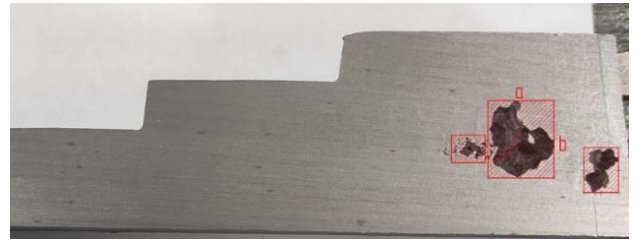
Fig. 13. Measurement of the area of shrinkage defects after cutting a stepped casting
