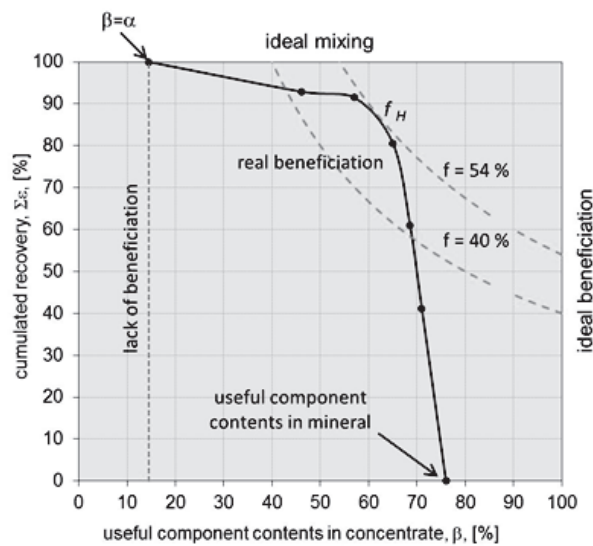
Fig. 1. Properties of Halbach's partition curve in system \varepsilon = f(\beta) , general data and location of point f_H , course of function f = \varepsilon\beta/100\% dependably on the value of f
