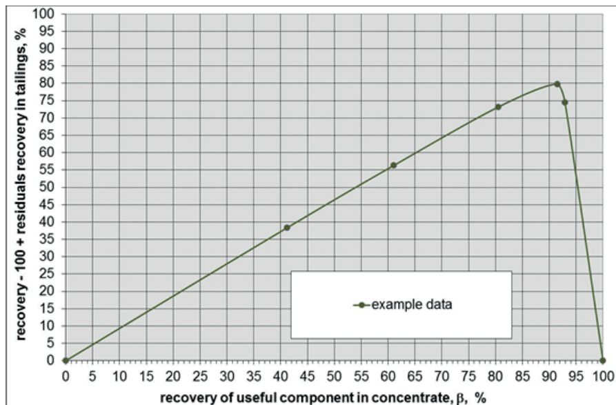
Fig. 5 Set of curves for ore beneficiation in system:
