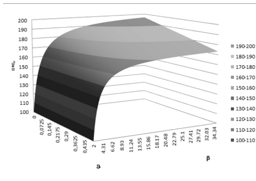
Fig. 4. Partition surface
