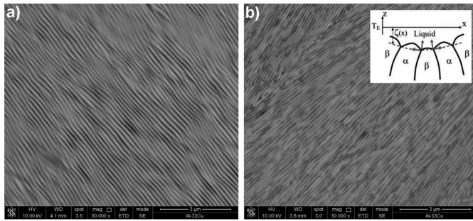
Fig. 5. Microstructures of \phi 3 mm Al-33Cu rod suction-cast at x = 27.5 mm: a) close to the rod surface, b) in the rod axis (SEM, 30000 \times ). Inset shows a schematic illustration of lamellar elimination caused by a concave perturbation of the eutectic front [17]
