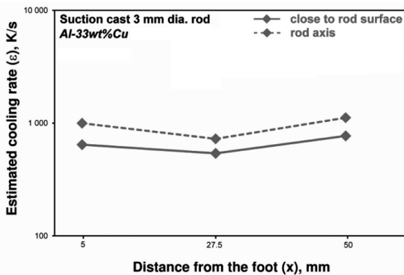
Fig. 6. Estimated superficial and axial cooling rates in Al-33wt%Cu ( \phi 3 \times 55 mm) suction cast alloy
