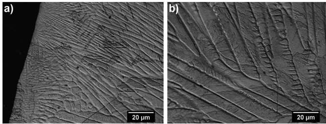
Fig. 3. Cross-sectional microstructure of the copper-mould cast \phi 3 mm Fe-25Ni alloy at x=5 mm: a) near the rod surface, b) in the rod axis (light microscopy, 1000x)
