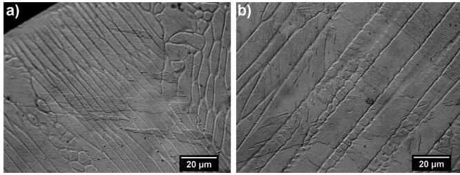
Fig. 2. Cross-sectional microstructure of the suction cast \phi 3 mm Fe-25Ni alloy at x=5 mm: a) near the rod surface, b) in the rod axis (light microscopy, 1000x)
