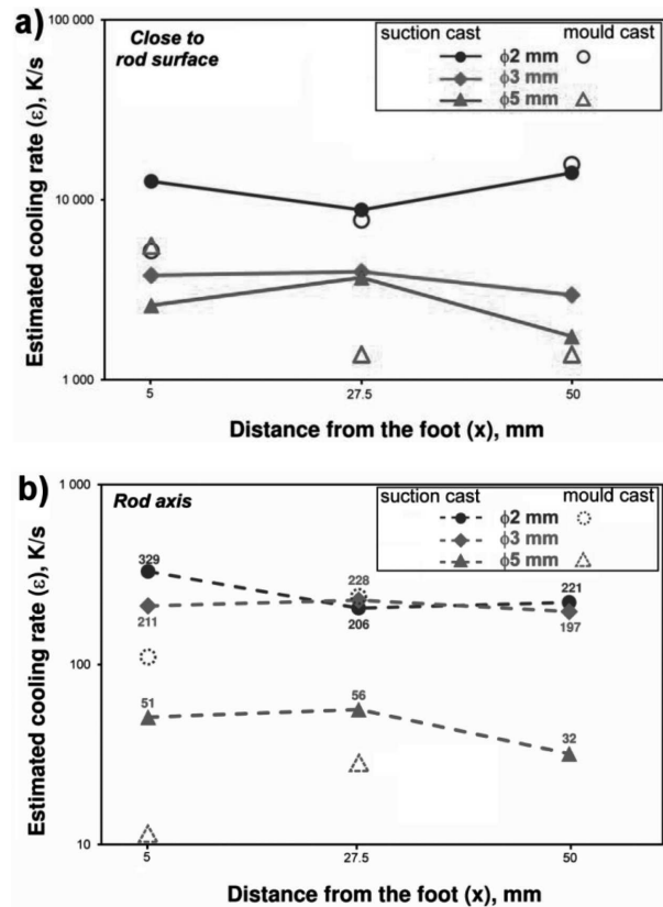
Fig. 4. Estimated a) superficial and b) axial cooling rates based on observed cellular spacing in Fe-25Ni alloy
