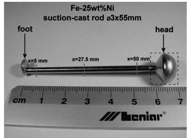
Fig. 1. A suction-cast \phi 3 \times 55 mm Fe-25Ni rod
