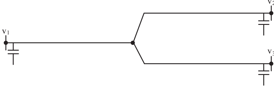
Fig. 30. Lumped parameter three-terminal line model
