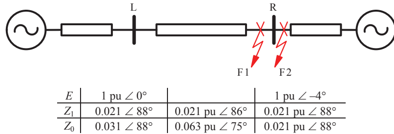
Fig. 14. Example power system
