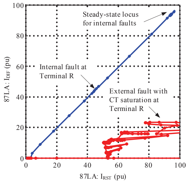
Fig. 24. Adding to the restraining signal terms corresponding to the difference between the rms and fundamental component currents enhances percentage differential element security
