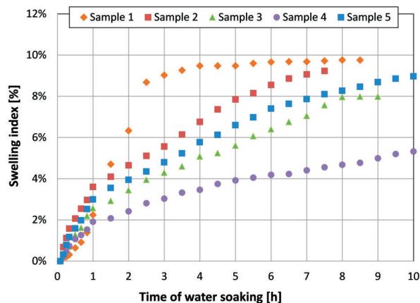
Fig. 8. The changes of swelling index in claystones from the Laziska Beds (Janina colliery)
