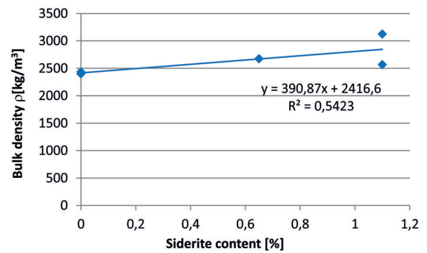
Fig. 13. The influence of siderite content on bulk density of claystones
