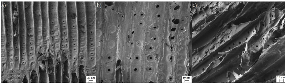
Fig. 2. SEM images of spruce wood samples: a – radial section of control sample, b – radial section of samples treated with Bioprep 3000 L, c – radial section of samples treated with Viscozyme L
