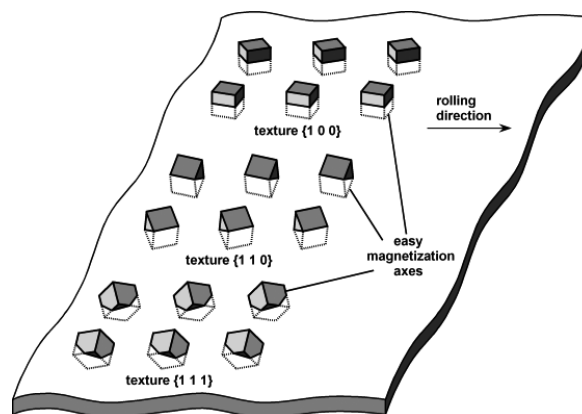
Fig. 2. Examples of the basic textures occurring in dynamo sheets
