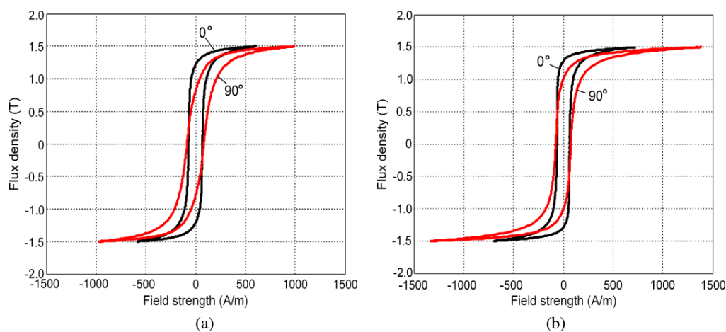
Fig. 1. Hysteresis loops of two different dynamo sheets measured along both the rolling and the transverse directions: M530-50A – South Korea (a); M530-50A – Czech Republic (b)
