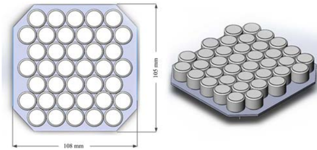
Fig. 2. Three-dimensional model of parametric array with 38 elements.
